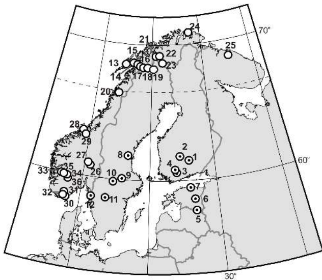
Fig. 1. The location of the sites from where the quantitative pollen-based temperature reconstructions were derived. The filled circles indicate sites with T_{\text{ann}} reconstructions and open circles with T_{\text{jul}} reconstructions. For the name of the sites, see Table 1.
