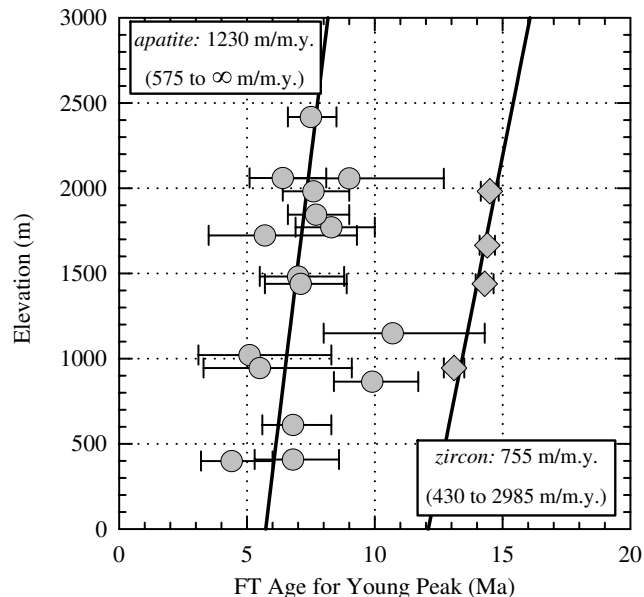
Figure 11. Age-elevation plot of fission-track (FT) minimum ages for apatite and zircon samples from the central massif. Error brackets ages show the 68% confidence interval. Regression lines were fit using weighted least squares (Press et al., 1992, p. 655–660). Errors were assumed to reside totally in the fission-track ages and weights were assigned using the age uncertainties. The estimated exhumation rate is equal to the inverse of the slope of the regression line and its uncertainty is calculated from the uncertainty for the estimated regression slope (Press et al., 1992, p. 657). This accounts for the asymmetric uncertainties for the estimated exhumation rates, the upper interval being much larger than the lower interval. Note that if the error brackets for the individual ages were extended to the 95% confidence interval, they would all overlap their respective best-fit line.
