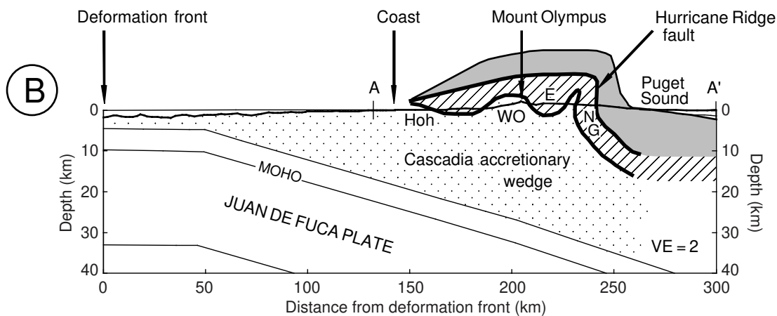
Figure 4. Generalized (A) geologic map and (B) cross section for the Olympic subduction complex (OSC). Numbers indicate minimum ages for apatite fission-track (FT) samples (Tables 1 and 2), and are considered to be reset ages for all MR, PR, or R samples (triangle, diamond, and circle, respectively). Bold outlines indicate localities with published zircon fission-track ages (right sides of Tables 1 and 2). The outer and inner ruled lines mark the base of the partial annealing zone for fluorapatite and \alpha -damaged zircon, respectively. Tectonostratigraphic units of Tabor and Cady (1978a) are shown as NG—Needles—Gray Wolf, E—Elwha, GV—Grand Valley, WO—Western Olympic, and Hoh.
