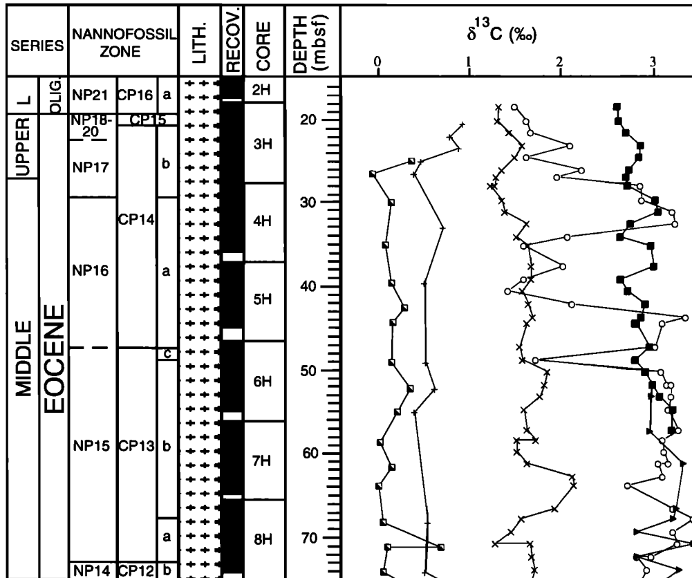
Figure 10. Planktonic and benthic foraminifer \delta^{13}\text{C} (‰ versus PDB) records of the lower to upper Eocene of Hole 865B. Planktonic taxa are separated into species, and benthic taxa are differentiated. See key in Figure 5 for symbols.
