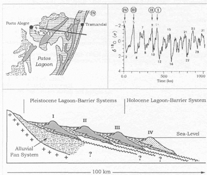
Figure 2-Generalized section of depositional systems across the coastal plain of Rio Grande do Sul. Barriers are correlated with the last peaks of oxygen isotopic curve (Williams et al 1988 - Fig 14). See Fig.1 for location and captions.
