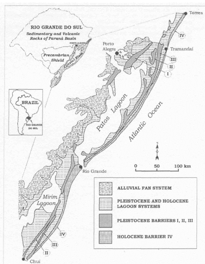
Figure 1-Location and simplified geologic map of Rio Grande do Sul coastal plain (Modified from Tomazelli and Villwock 1996).
