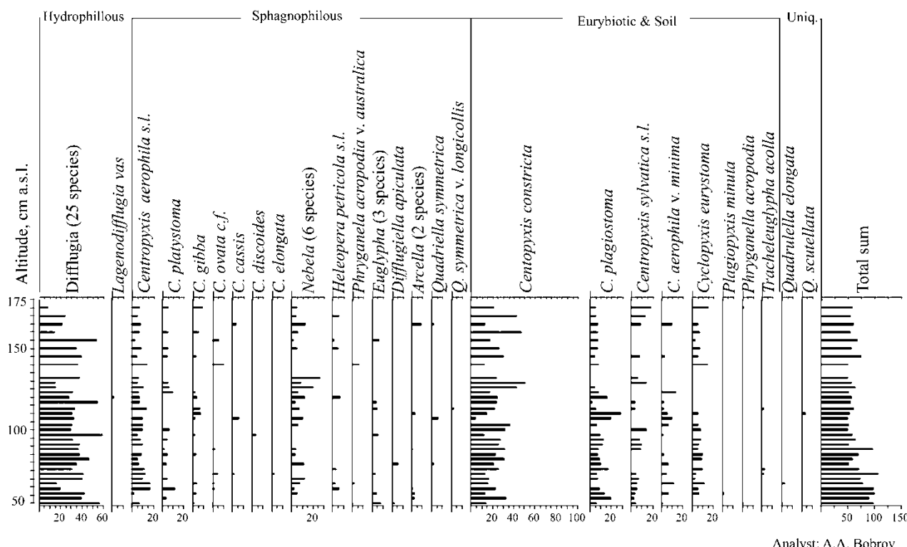
Fig. 6. Rhizopod percentage diagram of section R8+50.
