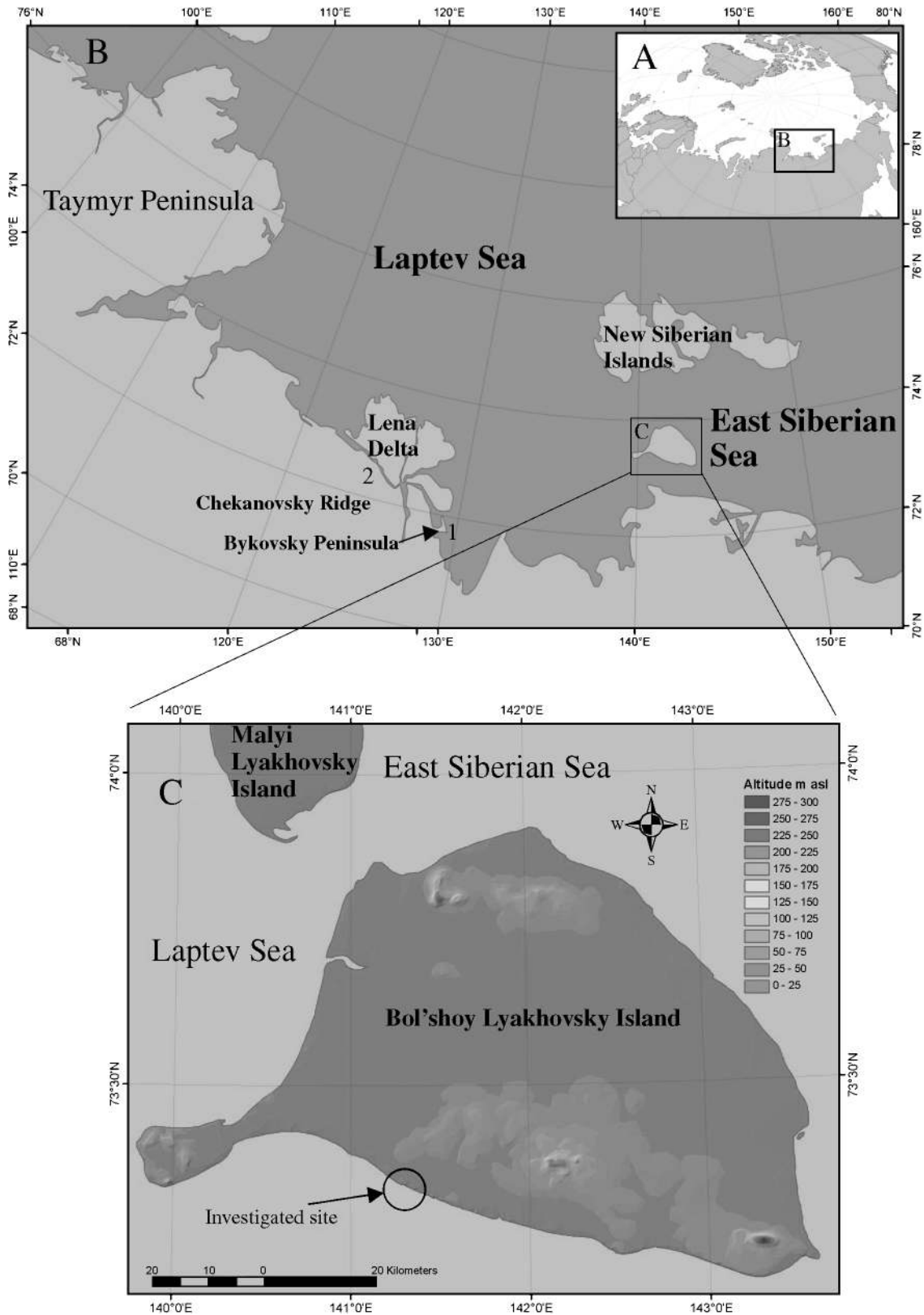
Fig. 1. A. Map of the Arctic. B. Map of the Laptev Sea – Bol'shoy Lyakhovsky Island region. 1 – Mamontovy Khayata site, 2 – Buor-Khaya site. C. Study area on Bol'shoy Lyakhovsky Island.
