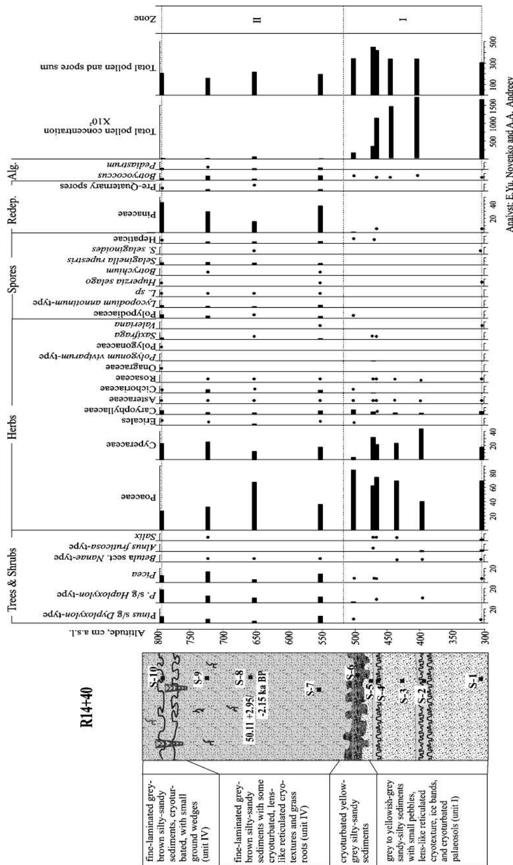
Fig. 7. Cryolithological structure and pollen percentage diagram of section R14+40 (for legend, see Fig. 3).
