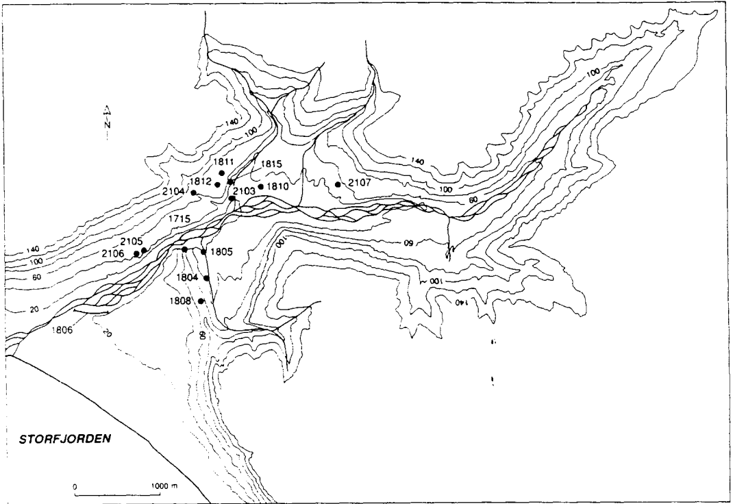
Fig. 7. Visdalen, showing the location of all sites described in the text.
