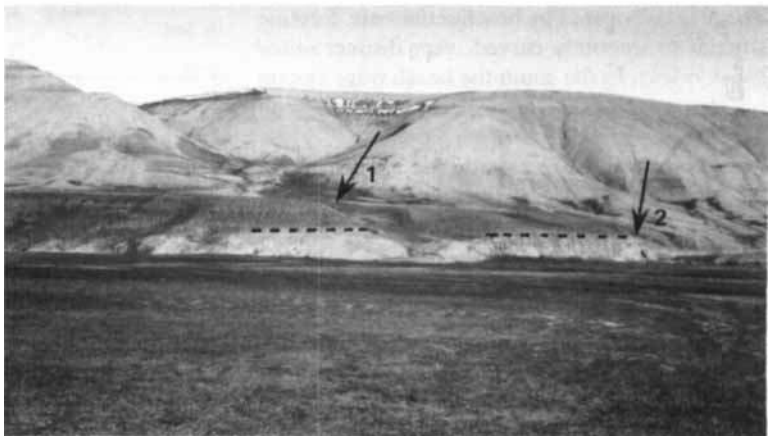
Fig. 6. The northern valley side around site 2104. The marine terrace has a fan-shaped overprint with the apex pointing towards a system of tributary valleys cut into the mountain in the north. Fine-grained glaciolacustrine sediments cling onto the coarse-grained sediments of the main terrace, demarcated with a dashed line. Site 2104 is shown by arrow (1) and site 2103 by arrow (2).
