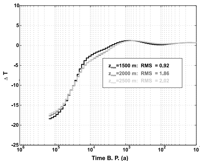
Figure 13. Comparison of inversions of truncated logs from the UDRYN borehole. The best fit could be obtained from the shortest logs. Data fit is measured by RMS = \sqrt{\frac{1}{N} \frac{(T_{obs} - T_{calc})^2}{\sigma^2}} .
