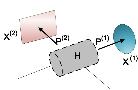
Figure 1: Illustration of multi-view latent representation. Observations \{\mathbf{X}^{(v)}\}_{v=1}^V ( V \geq 2 ) corresponding to different views are partially projected by \{\mathbf{P}^{(v)}\}_{v=1}^V from one underlying latent representation \mathbf{H} .
