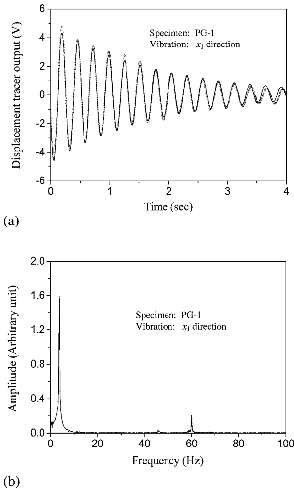
FIG. 3. (a) Time trace of the free vibration amplitude for PG-1. (b) Frequency spectrum of the PG-1 vibration.
