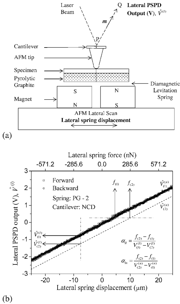
FIG. 4. (a) A schematic of the D-LFC. (b) A diagram showing the D-LFC principles for measuring the force constants \alpha_{||} and \alpha_{\perp} : the data set was collected with the PG-2 diamagnetic spring for the NCD AFM cantilever-bead assembly.
