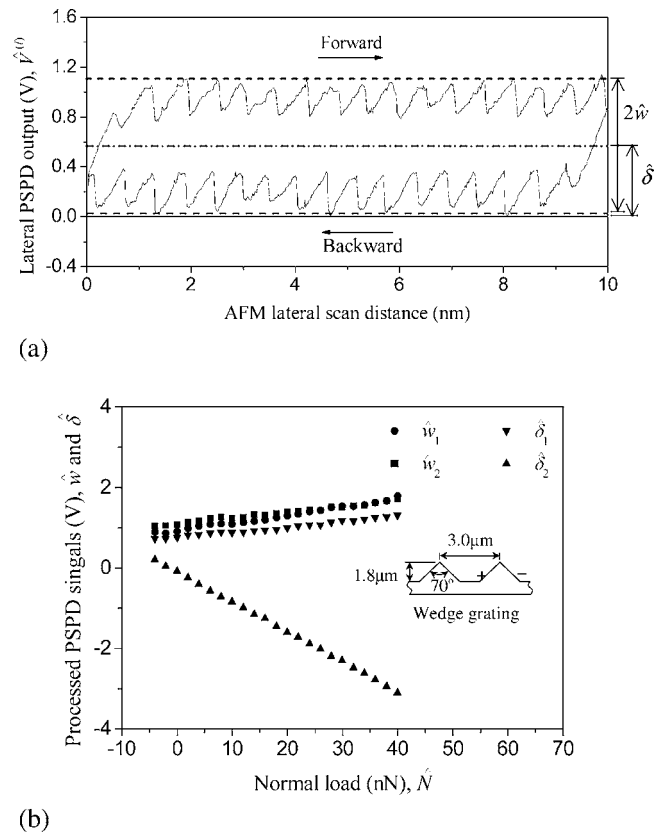
FIG. 6. (a) A friction loop of a contact B tip sliding on a mica surface: \hat{w} and \hat{\delta} denote the half-width and the central-value offset of the loop. (b) W-LFC data of \hat{w} and \hat{\delta} , which depend on the normal load for the NCC* tip sliding on the two different slopes of a wedge.
