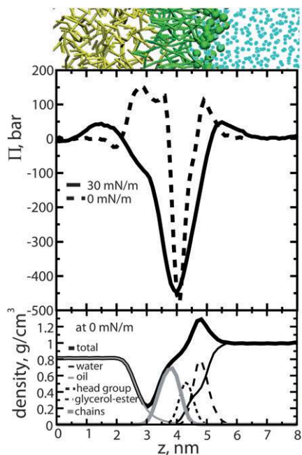
Fig. 2 Distribution of lateral pressure and density for a DPPC monolayer at the oil/water interface in the coarse-grained model. Lateral pressure profiles are shown at surface tensions of 0 and 30 mN/m, the partial density only at 0 mN/m. Lipids are shown as sticks, the head-group particles are marked as spheres, oil and water as in Fig. 1.
