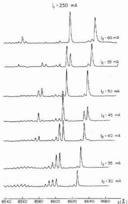
Fig. 5. Longitudinal mode spectrum of the device of Fig. 4 as a function of tuning current in cavity 2 (the long cavity).
