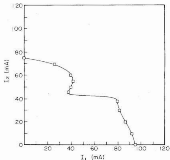
Fig. 6. Threshold gains of a device with D \approx 3 \mu\text{m} .
