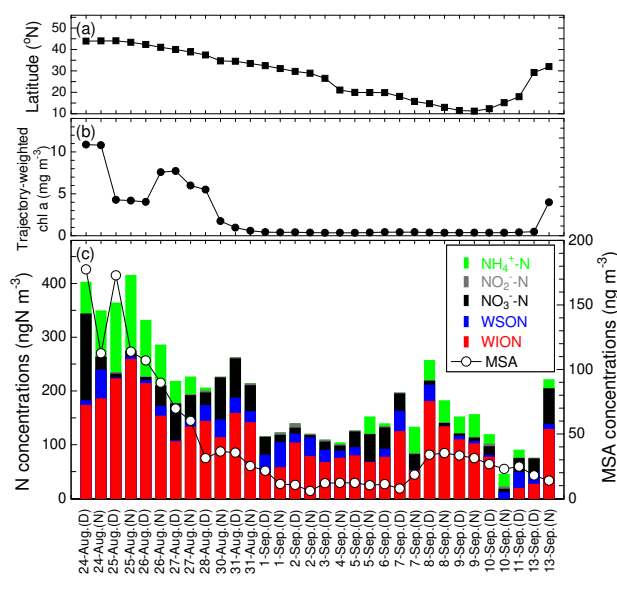
Fig. 3. Time series of (a) the average latitudinal location of the ship, (b) concentrations of trajectory-weighted chlorophyll- a and (c) fractions of organic (WSON and WION) and inorganic nitrogen together with concentrations of MSA. “D” means data obtained in daytime, whereas “N” means data obtained in nighttime.
