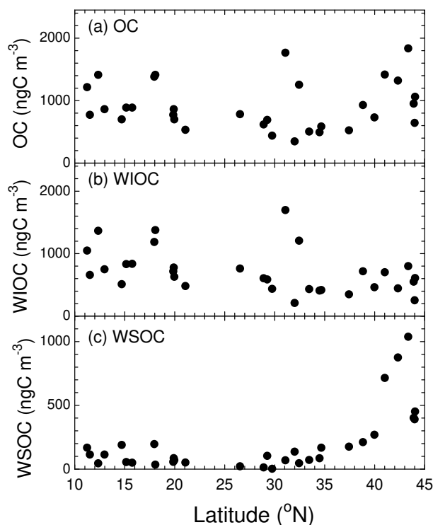
Fig. 5. Latitudinal distributions of (a) organic carbon (OC), (b) water-insoluble organic carbon (WIOC), (c) water-soluble organic carbon (WSOC).
