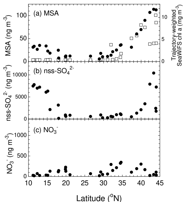
Fig. 2. Latitudinal distributions of MSA, \text{nss-SO}_4^{2-} , and \text{NO}_3^- . Also shown are 5-day back trajectory-weighted SeaWiFS chlorophyll- a concentrations as square symbol.
