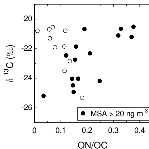
Fig. 6. Scatter plots between \delta^{13}\text{C} and ON/OC ratios. Solid circles indicate the data with \text{MSA} > 20\ \text{ng m}^{-3} .
