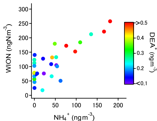
Fig. 8. A linear relation between WION and \text{NH}_4^+ , color-coded according to the concentration of \text{DEA}^+ .
