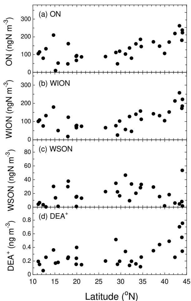
Fig. 4. Latitudinal distributions of (a) organic nitrogen (ON), (b) water-insoluble organic nitrogen (WION), (c) water-soluble organic nitrogen (WSON), and (d) diethylammonium ( \text{DEA}^+ ).
