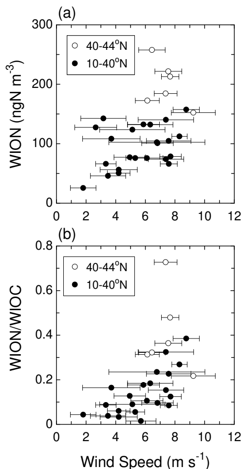
Fig. 7. Relations of (a) WION concentrations and (b) WION/WIOC ratios with local wind speed at 40–44° N (open circles) and 10–40° N (solid circles). Values and bars for wind speed indicate averages and standard deviations, respectively, during each sampling time.
