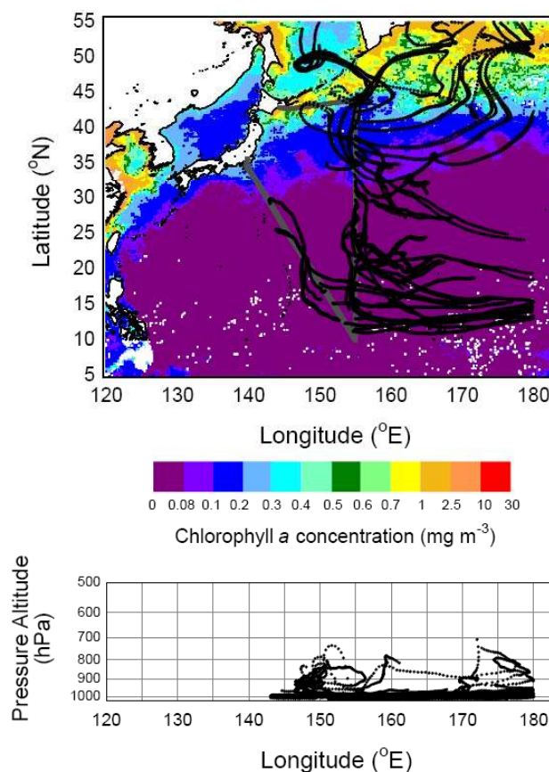
Fig. 1. R/V Hakuho cruise track in the western North Pacific between 24 August and 13 September 2008, together with typical 5-day back trajectories. Also shown are monthly averaged concentrations of chlorophyll- a for August–September 2008 derived from SeaWiFS data, available from the NASA Goddard Space Flight Center/Distributed Active Archive Centers. A white dot indicates that the satellite data is missing at a corresponding grid.
