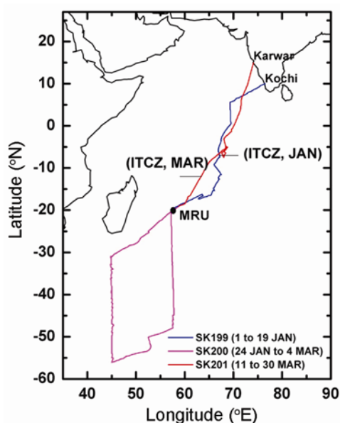
Figure 1. Cruise tracks for SK199, SK200 and SK201.
