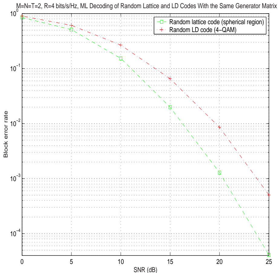
Figure 1: Random LAST code versus random LD code.
