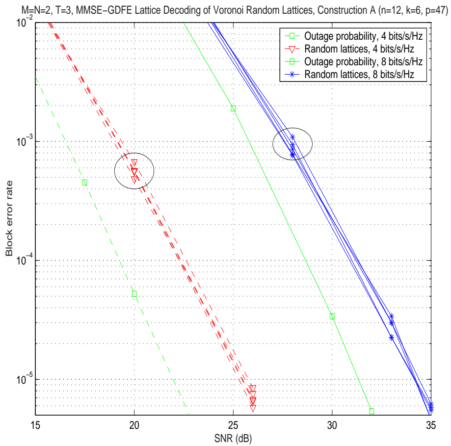
Figure 3: Random nested LAST codes with MMSE-GDFE lattice decoding achieve the optimal diversity-vs-multiplexing tradeoff.
