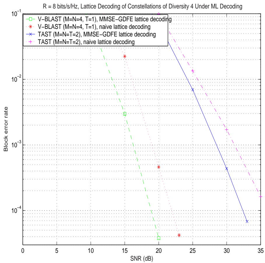
Figure 2: MMSE-GDFE lattice decoding versus naive lattice decoding.
