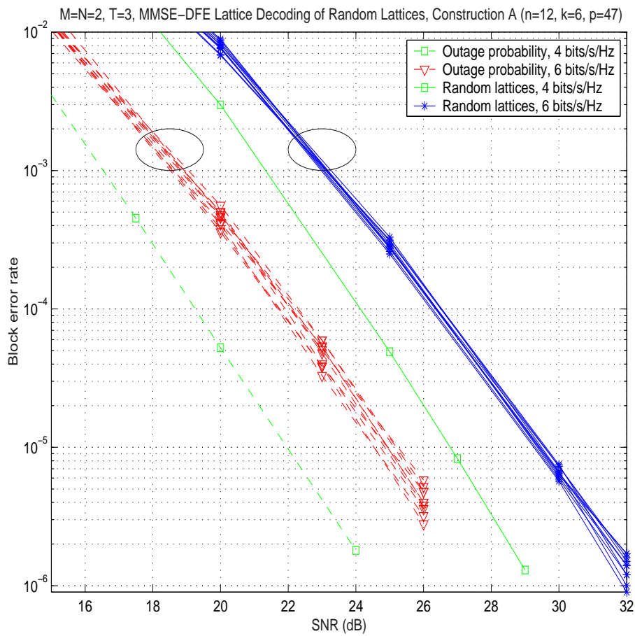
Figure 4: Random spherical LAST codes with MMSE-GDFE lattice decoding achieve the optimal diversity-vs-multiplexing tradeoff.
