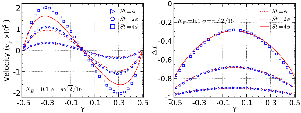
FIGURE 6. The velocity and temperature perturbations ( \Delta T ) for a hard-sphere gas subject to a sinusoidal heating at t = 3\pi/2 at different Kn and St. The symbols correspond to the data of the lattice model ( Pr = 2/3 ) and the lines are the results of the LVDSMC method.
