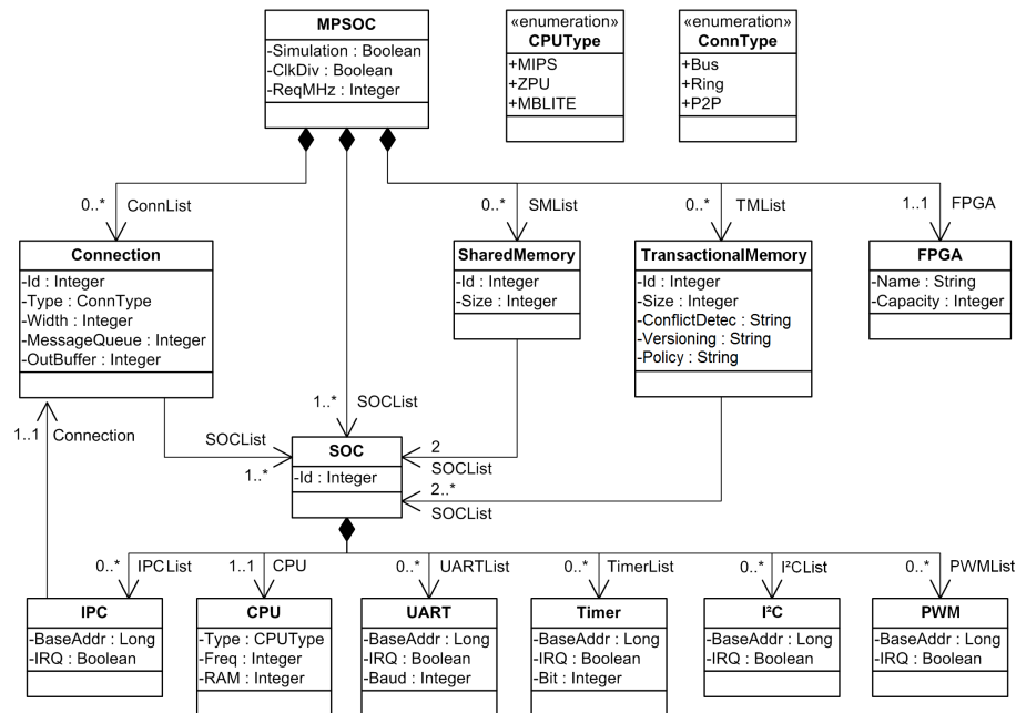
Figure 1: Excerpt from the LavA meta model
