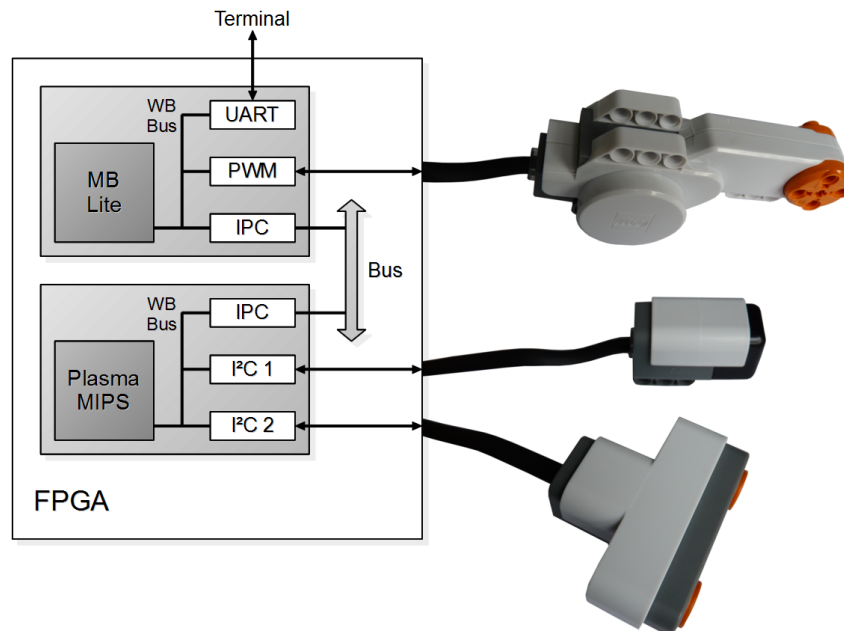
Figure 2: Multiprocessor system with connected Lego Mindstorms NXT sensors and actuators
