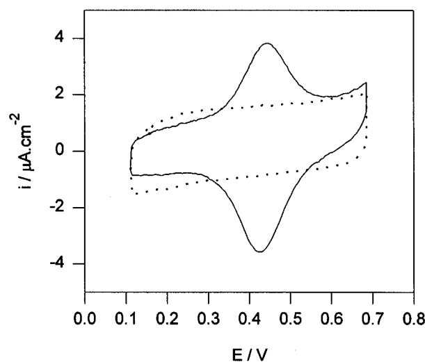
Figure 5. Cyclic voltammogram of Au with 3-mercaptopropanesulfonate SAM (···) and Au/Thiol with Fc-PAA SAM in 10 mM acetic/acetate buffer of pH 5.0 (—). Sweep rate: 50 \text{ mV s}^{-1} . (a) Au/thiol; (b) Au/thiol/PAA-Fc. Ferrocene charge: 6.5 \mu\text{C cm}^{-2} .
