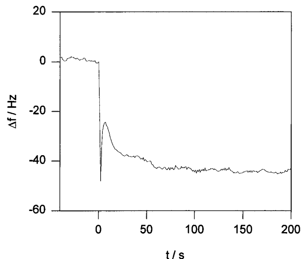
Figure 3. Time dependence of the quartz crystal resonance frequency shift for the adsorption of 3-mercaptopropanesulfonate on Au from 0.02 mM thiol solution in 0.01 mM \text{H}_2\text{SO}_4 . Measurements were made using a 10 MHz AT-cut quartz crystal with an areal mass sensitivity of 0.229 \text{ Hz cm}^2 \text{ ng}^{-1} .
