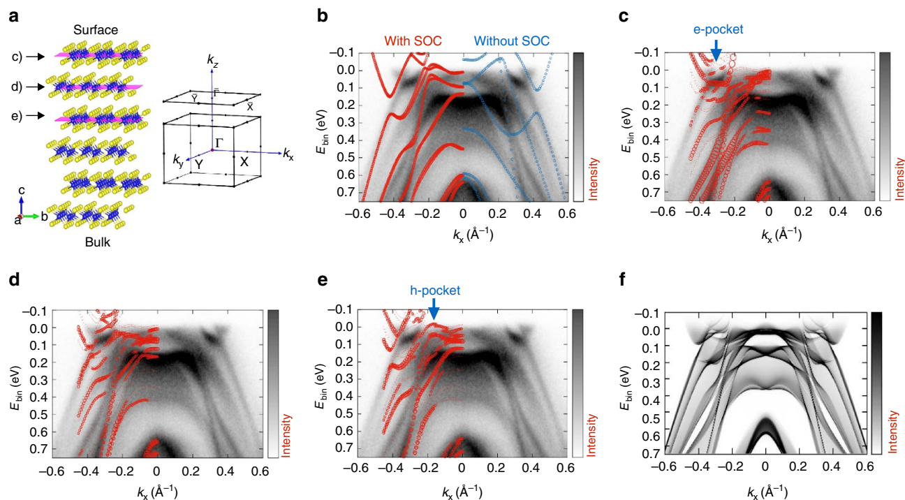
Figure 2 | Evolution of band structure with number of layers. (a) Crystal structure of \text{WTe}_2 with the bulk and surface Brillouin zones on the right. On the left, the slab model used in the theoretical calculations, consisting of six Te-W-Te layers; each layer is formed by hexagonally packed W sandwiched between two Te layers. (b–e) ARPES measurements ( h\nu = 68 eV, T = 77 K) of the electronic structure along the \Gamma\text{X} high symmetry direction (along the W chains); (b) bulk electronic structures as calculated with SOC (red bands at negative momenta) and without SOC (blue bands at positive momenta); (c) theoretical bands projected on the topmost \text{WTe}_2 planes; (d, e) theoretical bands projected on second and third plane, respectively. In c, e, blue arrows mark the positions of the theoretical electron and hole pockets, respectively. In b, e, the size of the circles is proportional to the weight of the layer-resolved orbital character, calculated as the sum of the orbital characters of all the atoms belonging to the respective layer. (f) The theoretical surface spectral function A(\mathbf{k}, E) .
