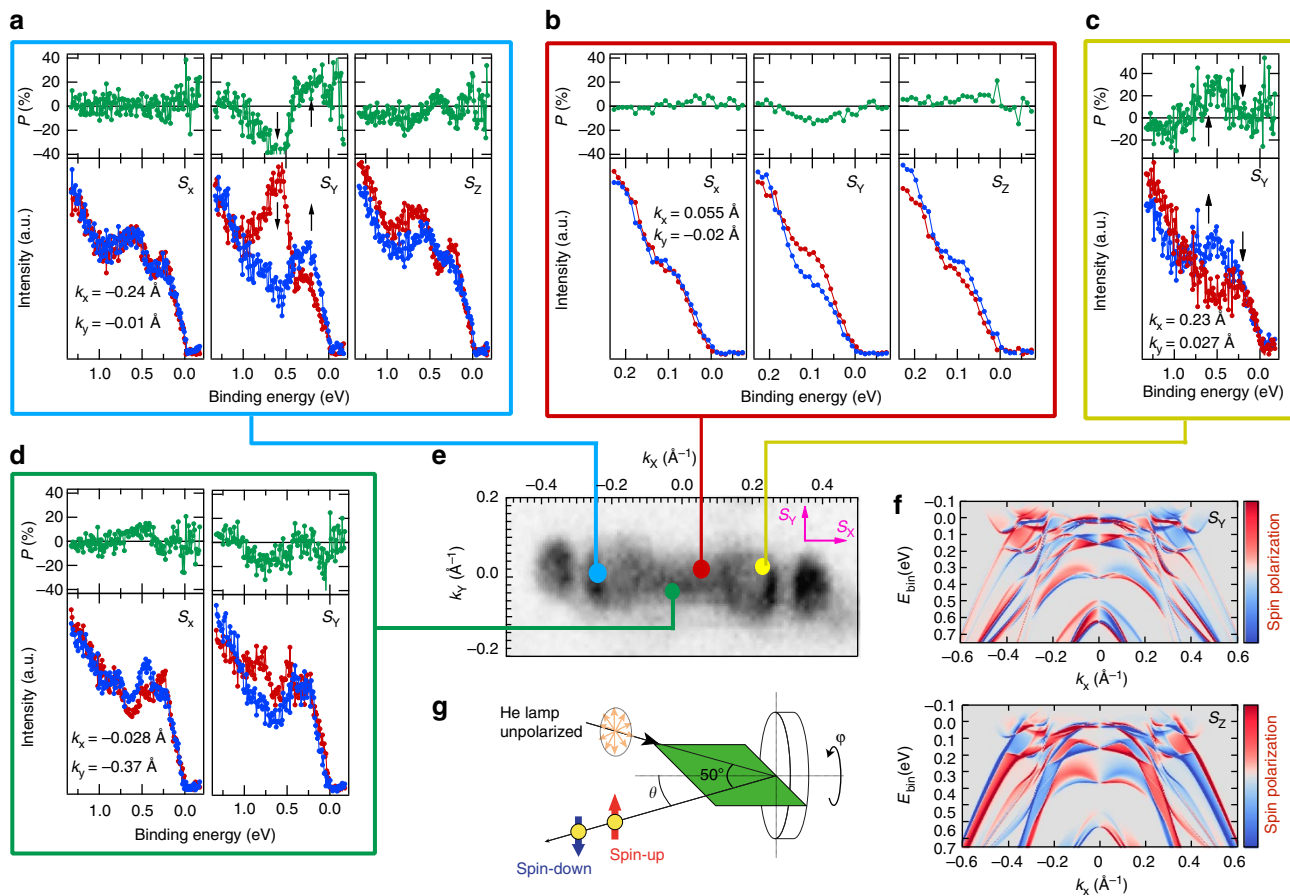
Figure 4 | Experimental and theoretical spin polarized band structure of large SOC and non-centro-symmetric WTe_2 . (a–d) Measured spin-resolved ARPES spectra (red and blue curves) and spin polarization (green curves) at four distinct \mathbf{k} points as indicated in e; (e) experimental Fermi surface with the corresponding spin measurement positions; (f) calculated band structure along k_x direction, upper/lower panel shows S_y/S_z spin orientation. The colour scales represent the degree of spin polarization; red, blue and white refer to up, down and no-spin polarization, respectively; (g) experimental geometry of spin-resolved ARPES setup. In a, S_y , the down-spin spectrum (red curve) has a larger peak at 0.6 eV (down arrow) and the up-spin spectrum (blue curve) has a larger peak at 0.2 eV (up arrow), whereas at c, on the contrary, the up-spin spectrum has a dominating peak at 0.6 eV and the down-spin spectrum has a dominating peak at 0.2 eV, supporting time-reversal effect.
