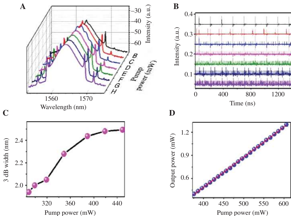
Figure 6: Output signals with the power of the pump increasing. (A) The spectrum evolution versus the pump power. (B) The pulse train evolution versus the pump power. (C) The 3-dB spectral width versus the pump power. (D) Output power and linear fitting slope curve versus pump power.
