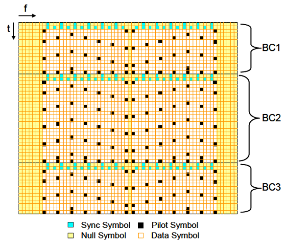
Figure 9. Structure of the Broadcast Frame
