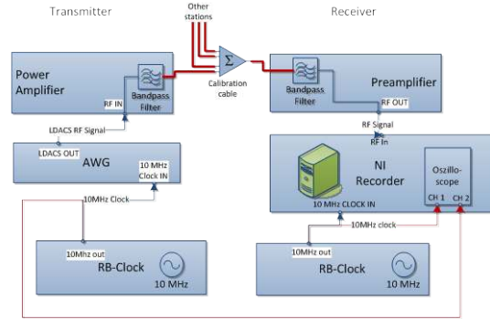
Figure 7. Calibration Setup for a Single Station
