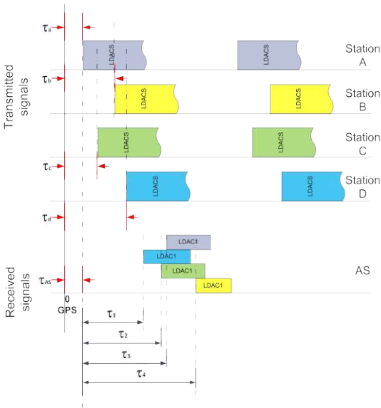
Figure 6. Calibration of the Measurement Setup
