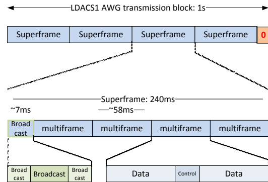
Figure 8. Structure of the Transmitted LDACS1 Signal
