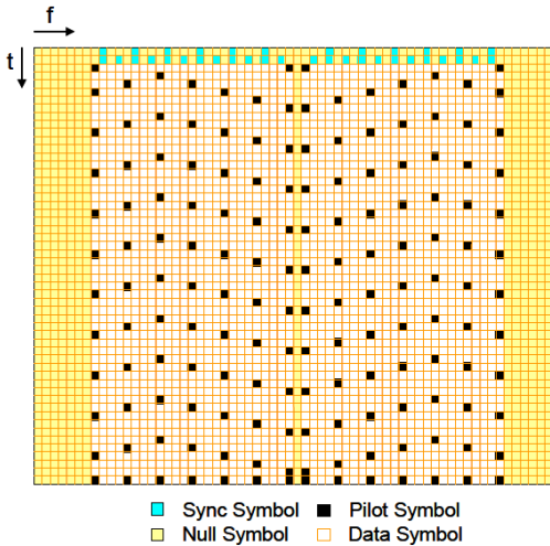
Figure 10. Structure of the Data/Control Frame
