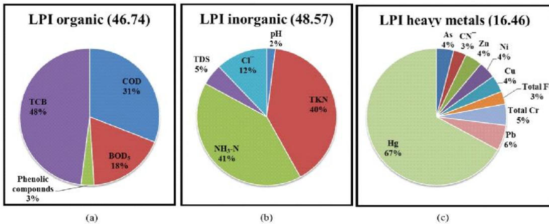
Fig. 3: Percentage distribution of the components of (a) LPI organic, (b) LPI inorganic and (c) LPI heavy metals for the closed dumping ground at Dhapa, Kolkata
