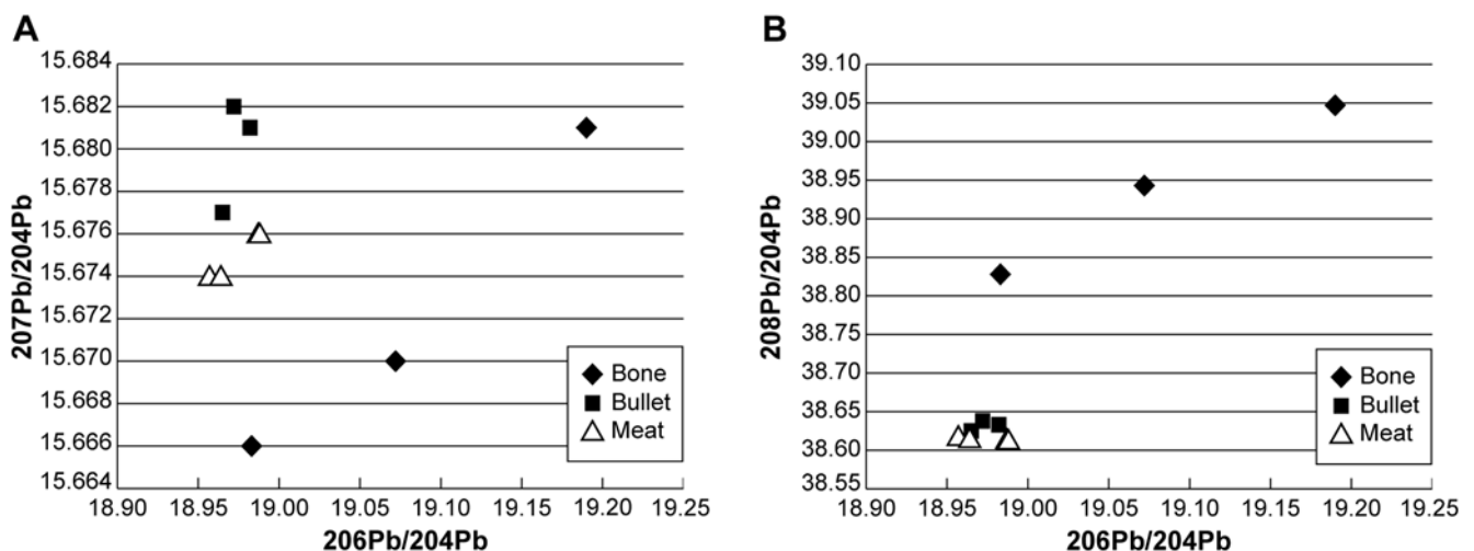
Figure 1. Plots of lead isotope ratios in ground meat samples containing radiodense fragments from four deer. Ratios from lead-in-meal samples clustered with those of unfired bullets but were distinct from bone lead ratios. Note that there are four meat data points (open triangles) in each graph, but two have almost identical positions and are superimposed. doi:10.1371/journal.pone.0005330.g001
