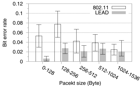
Figure 10: Effect of packet size on the bit error rates of 802.11 and LEAD.
