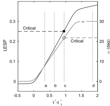
Fig. 3 Pitch angle variation, and LESP history from inviscid theory for the baseline case. The four times instants marked ( a–d ) are used to discuss LEV initiation. The LESP value at instant ( c ) corresponding to LEV initiation from CFD is termed the critical LESP. This critical LESP and the corresponding \alpha are marked in the figure
