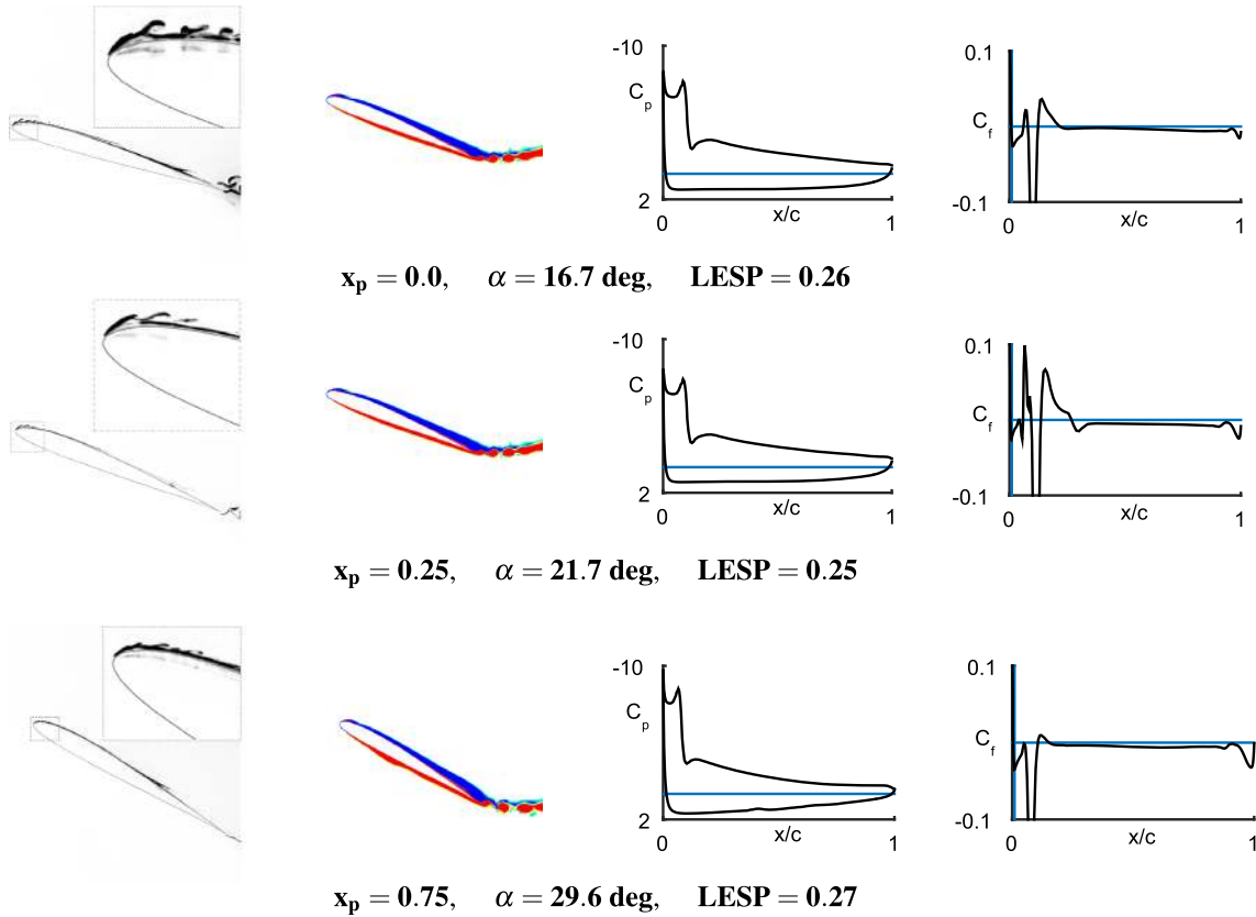
Fig. 8 Case study 1, effect of pivot location, at the instants of LEV initiation: left to right —flow visualization from experiment, vorticity plots from CFD, C_p ( upper and lower surfaces ) and C_f ( upper surface ) distributions from CFD
