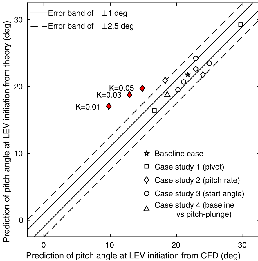
Fig. 22 Pitch angle at the instant of LEV initiation : x-axis shows predictions from CFD and y-axis shows prediction from theory using \text{LESP}_{crit} = 0.25 . The three red symbols indicate outliers (color figure online)
