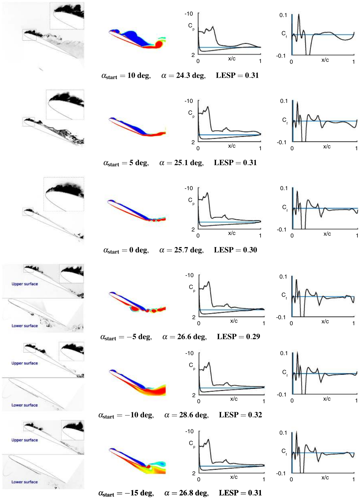
Fig. 17 Case study 3, effect of initial pitch angle, at \Delta LESEP = 0.05 after the instants of LEV initiation: left to right —flow visualization from experiment, vorticity plots from CFD, C_p ( upper and lower surfaces ) and C_f ( upper surface ) distributions from CFD
