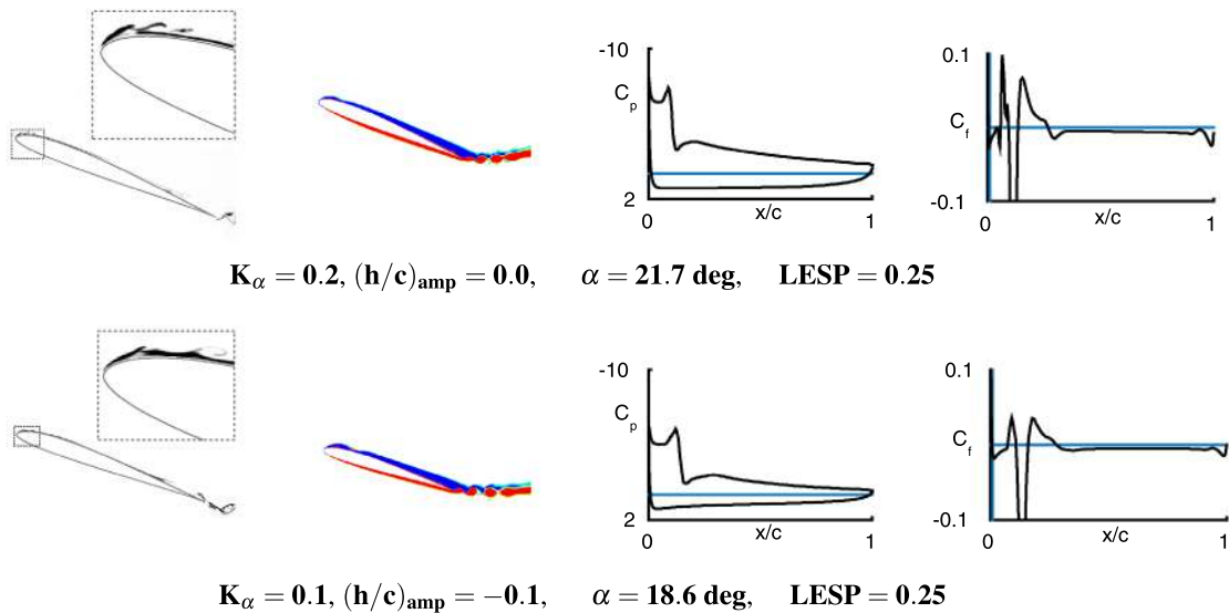
Fig. 20 Case study 4, baseline versus pitch–plunge combination, at the instants of LEV initiation: left to right —flow visualization from experiment, vorticity plots from CFD, C_p ( upper and lower surfaces ) and C_f ( upper surface ) distributions from CFD
