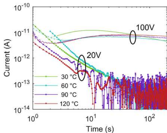
FIG. 3. Current transients during a reverse bias stress of 20 V and 100 V over a temperature range of 30\text{--}120^\circ\text{C} . The transients are only weakly temperature dependent with no trend emerging.
