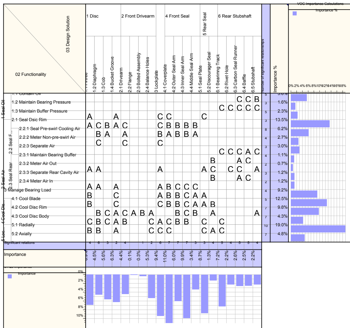
Figure 6.19: Completed QFD2 Showing Functional Importance, Relationship between Features and Functionality and Resultant Feature Importance
