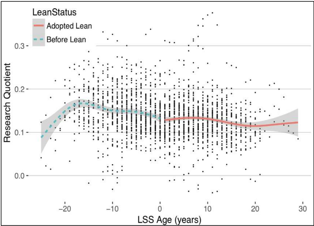
Figure 4-3: LSS Age vs. RQ
