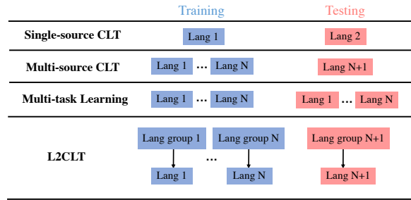
Figure 2: Differences between our work and other existing methods. “Lang” refers to the language.
