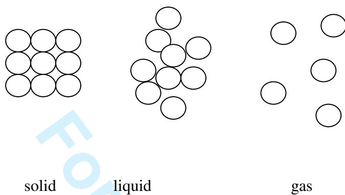
Figure 3. A representation of matter in the three different forms (after Henriksson 2004)
