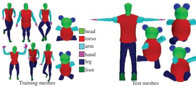
Figure 8: Merging categories. A CRF was learned from the training meshes on the left, which include both humans and teddy bears. Results on a test human and bears shown on right.
