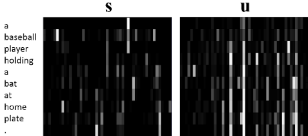
Figure 2. Illustration of the hidden units s and u activations through time (vertical axis). Notice that the visual hidden units u exhibit long-term memory through the temporal stability of some units, where the hidden units s change significantly each time step.
