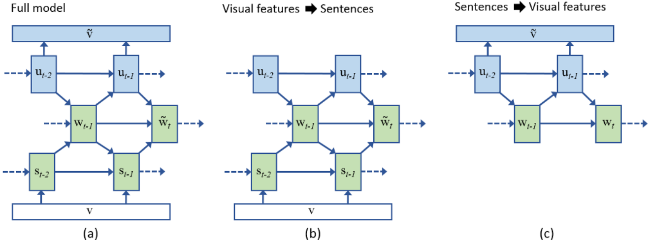
Figure 1. Illustration of our model. (a) shows the full model used for training. (b) and (c) show the parts of the model needed for generating sentences from visual features and generating visual features from sentences respectively.
