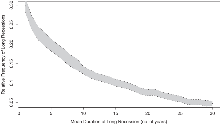
Figure 1. Relative frequency of long recessions: international evidence. Notes: The figure uses the international consumption data from Barro and Ursua (2012) as described in more detail in the Supplementary Appendix A.2. The confidence bounds correspond to percentile intervals from bootstrap with a random block length having geometric distribution.
