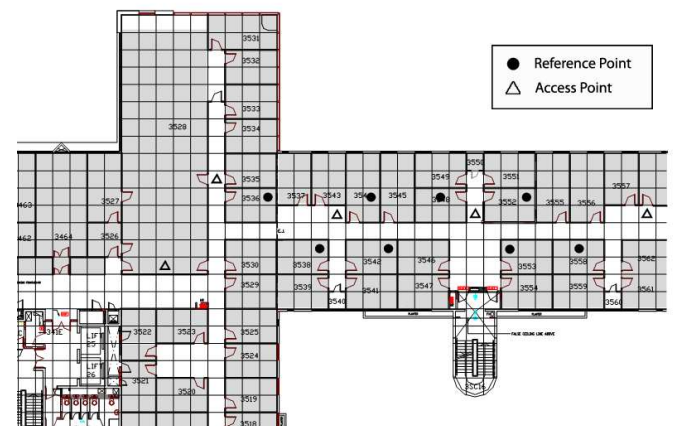
Fig. 6. The layout of the experimental test-bed
