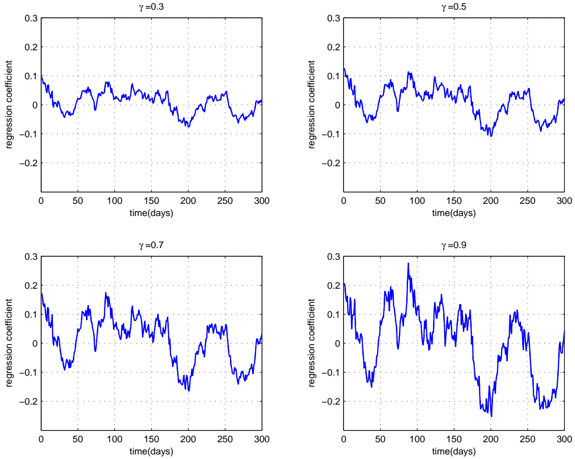
Figure 9. Regression analysis. For different parameters \gamma = 0.3, 0.5, 0.7, 0.9 we plot the time variation of the estimated parameter b in (49) for a rolling regression of R on \sigma_R^2 . The rolling regressions are based on sample sizes of 50 observations simulated from a model with three reference model drift states \Theta = \{0.0025, 0.0175, 0.0325\} and under an homogenous degree of ambiguity \eta = 0.01 . The true dividend is \theta = 0.0175 . Further parameters are \delta = 0.05 , \sigma_D = 0.0375 , \sigma_e = 0.015 .
