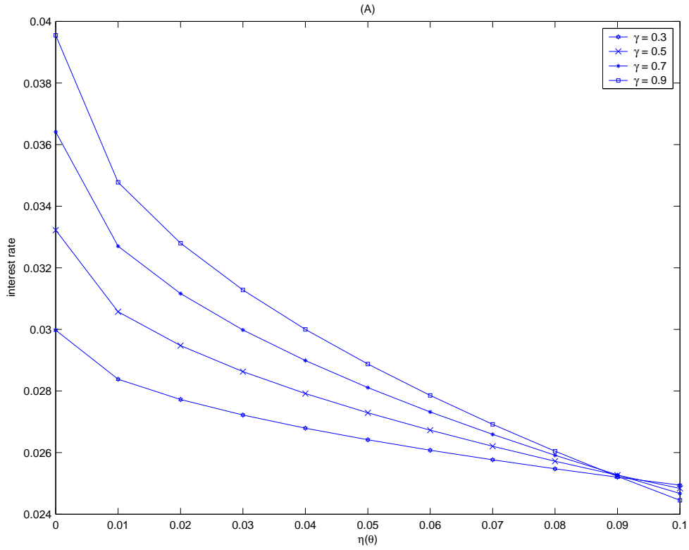
Figure 5. The equilibrium interest rate. We plot the equilibrium interest rate as displayed in Proposition 9 for different homogenous degrees of ambiguity \eta(\theta) and different risk aversions \gamma = \{0.3, 0.5, 0.7, 0.9\} . We assume five states \Theta = \{-0.0125, 0.0025, 0.0175, 0.0325, 0.0475\} and set \delta = 0.025 , \sigma_D = 0.0375 , \sigma_e = 0.015 with a constellation of discretized normal priors \Pi = \{0.0668, 0.2417, 0.3829, 0.2417, 0.0668\} .
