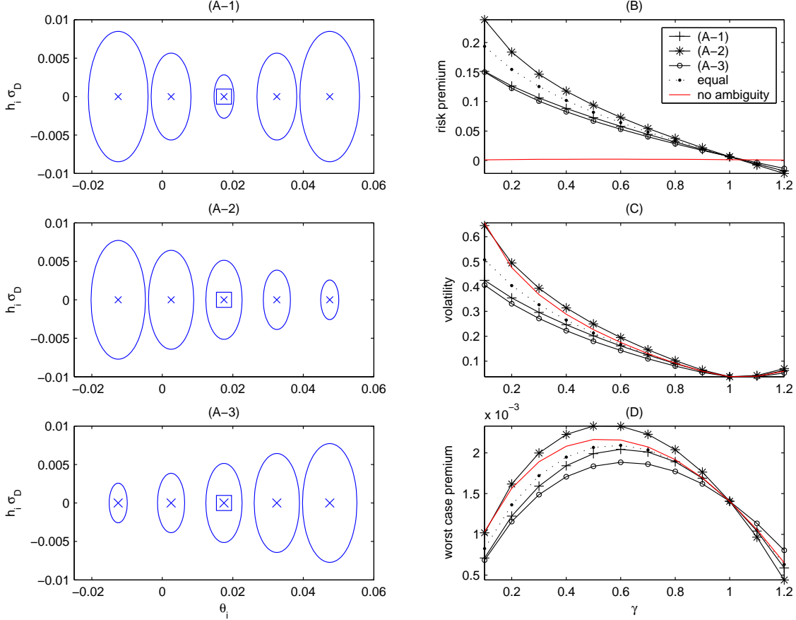
Figure 8. Panels (A-1)–(A-3) plot different entropy preserving distributions of ambiguity around the reference model dividend drift states \theta_1, \dots, \theta_5 , i.e., Panels (A-1)–(A-3) are such that the weighted entropy measure \frac{1}{2} \sum \pi_i h^2(\theta_i) is equal to 0.01, as in Figure 7. For Panel (A-1), we set \eta(\theta_i)_{i=1, \dots, 5} = \{0.0256, 0.0114, 0.0028, 0.0114, 0.0256\} , for Panel (A-2), \eta(\theta_i)_{i=1, \dots, 5} = \{0.0212, 0.0147, 0.0094, 0.0053, 0.0024\} and for Panel (A-3), \eta(\theta_i)_{i=1, \dots, 5} = \{0.0024, 0.0053, 0.0094, 0.0147, 0.0212\} . The set \Pi = \{0.0668, 0.2417, 0.3829, 0.2417, 0.0668\} of prior distributions and the set \Theta = \{-0.0125, 0.0025, 0.0175, 0.0325, 0.0475\} of reference model drifts relevant for all graphs are the same as those in Panel (A) of Figure 7. Panels (B), (C), and (D) plot, the equity premium \mu_R , the volatility \sigma_R and the worst case premium \mu_R^{wc} implied by the different distributions of ambiguity in Panels (A-1)–(A-3). For comparison, we plot in each graph the corresponding quantities prevailing under an homogenous (equal) ambiguity parameter \eta = 0.01 and in the absence of ambiguity ( \eta(\theta_i) = 0, i = 1, \dots, n ). Further parameters are \delta = 0.05 , \sigma_D = 0.0375 and \sigma_e = 0.015 .
