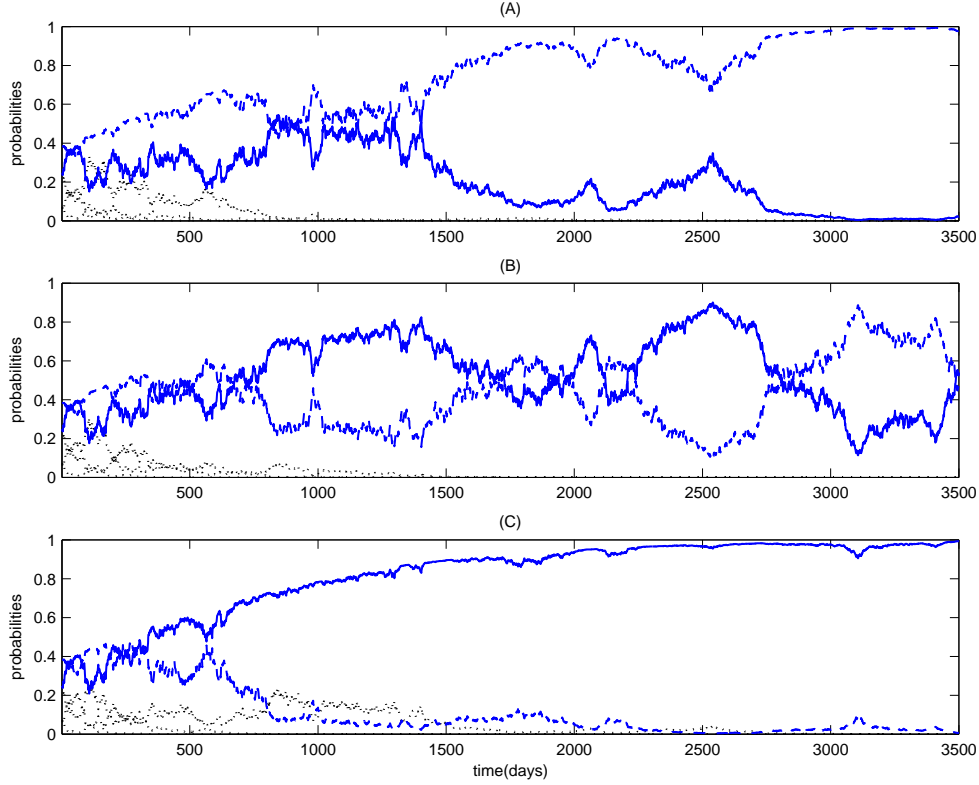
Figure 2. Posterior probabilities dynamics. Panels (A), (B), (C) plot for different random seeds the dynamics of the implied posterior probabilities when the learning model allows for five possible dividend drift states and the underlying dividend drift process is geometric Brownian motion with drift \theta_2 . In Panel (A), we assume that there is no likelihood misspecification, i.e., h(\theta_i) = 0 . In Panel (B), we introduce a simple (constant) misspecification and set h(\theta_i) = 0.141 , i = 1, \dots, n . In Panel (C), we increase the size of such misspecification to h(\theta_i) = 0.316 , i = 1, \dots, n . It turns out that the learning dynamics in Panels (A), (B), and (C) differ substantially. In Panel (A), state \theta_2 will eventually be correctly learned (see the dashed line in the graph). In Panel (B), the posterior probabilities does not converge after 3600 days. In Panel (C), state \theta_3 will be eventually "learned" (see the solid line in the graph). Model parameters are \Theta = \{-0.0125, 0.0025, 0.0175, 0.0325, 0.0475\} , \sigma_D = 0.0375 , \sigma_e = 0.015 , h_D = 0 .
