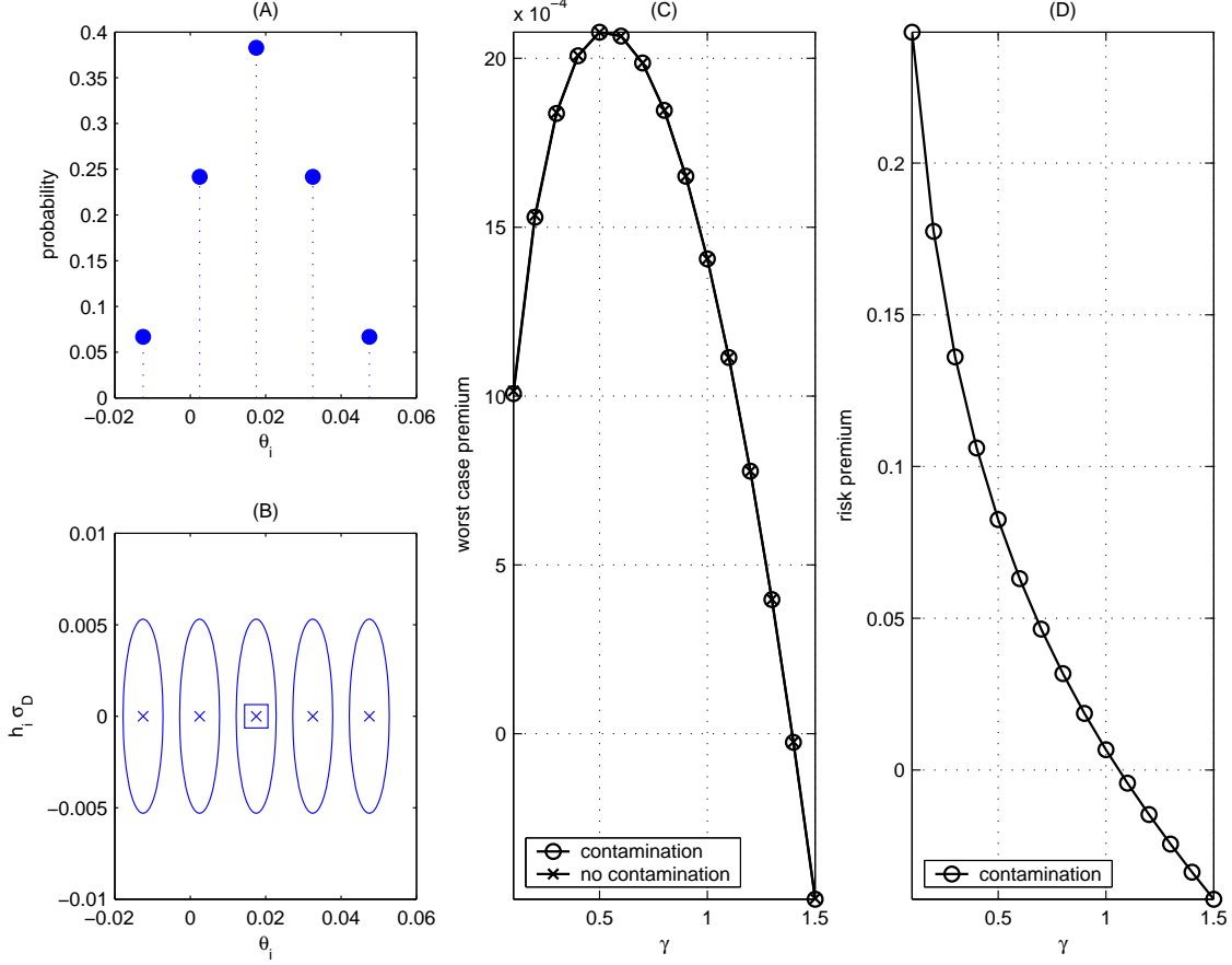
Figure 7. Panel (A) plots the set of probabilities \Pi relevant for the figure while Panel (B) plots the different relevant reference model states \theta_1, \dots, \theta_n . The true reference model dividend drift state is marked with a square and has been set equal to the posterior expected value \sum \pi_i \theta_i . We use a small amount of homogenous ambiguity \eta = 0.01 . The size of the ambiguous neighborhoods \Xi(\theta_1), \dots, \Xi(\theta_n) is highlighted by the ellipses centered at \theta_1, \dots, \theta_n in Panel (B). Further, we set \delta = 0.05 , \sigma_D = 0.0375 and \sigma_e = 0.015 . With these parameters the resulting worst case equity premium \mu_R^{wc} and the actual equity premium \mu_R are plotted in Panel (C) and (D) as functions of \gamma .
