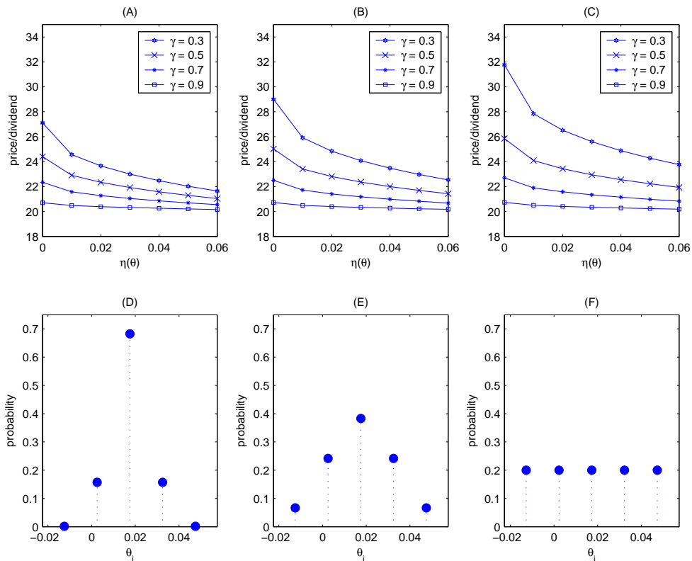
Figure 4. The impact of uncertainty and ambiguity aversion on price dividend ratios. In Panels (A)-(C) we explore the impact of mean preserving spreads on price dividend ratios. We display the prior distribution corresponding to each of those panels in the Panels (D)-(F). Given such prior distributions, we assume a setting with five possible states \Theta = \{-0.0125, 0.0025, 0.0175, 0.0325, 0.0475\} . We further set \delta = 0.05 , \sigma_D = 0.0375 , \sigma_e = 0.015 .
