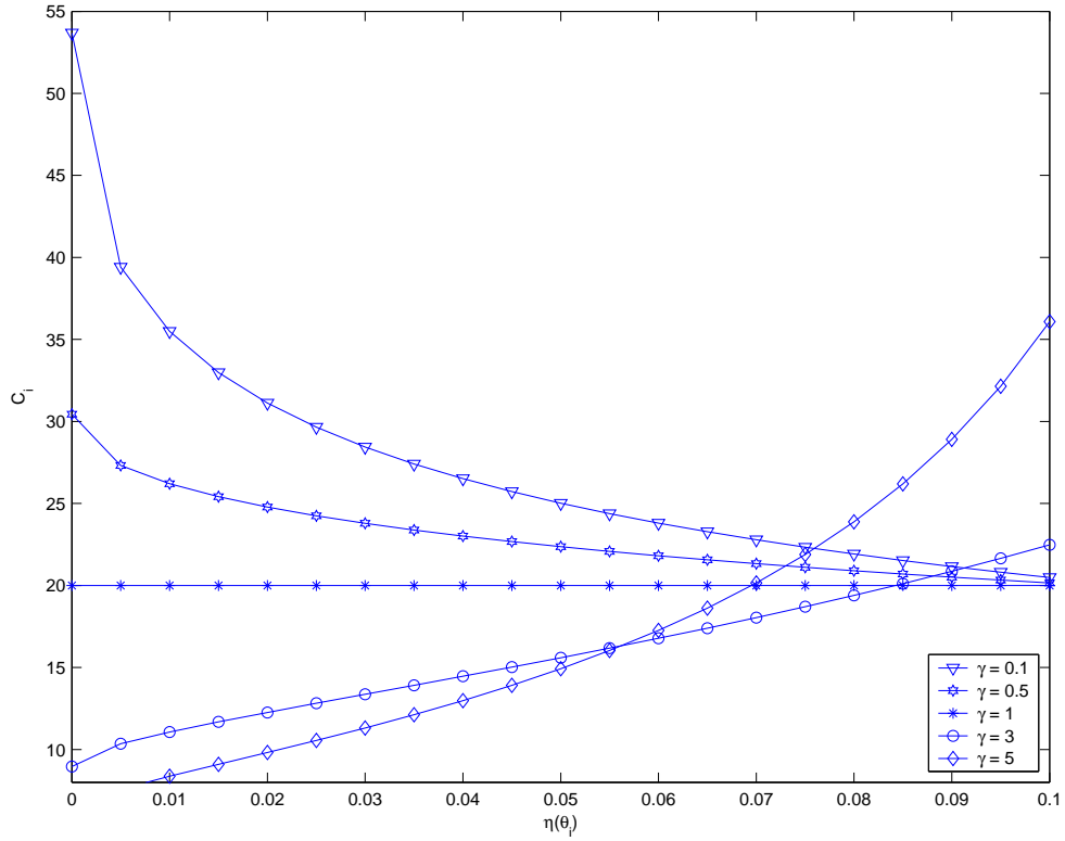
Figure 3. Function C_i in dependence of the ambiguity and risk aversion parameters \eta_i(\theta_i) and \gamma . We assume \delta = 0.025 , \theta_i = 0.0175 , \sigma_D = 0.0375 , and calculate C_i for different amounts of ambiguity, \eta_i(\theta_i) \in [0, 0.1] , and different degrees of risk aversion, \gamma = \{0.1, 0.5, 1, 3, 5\} .
