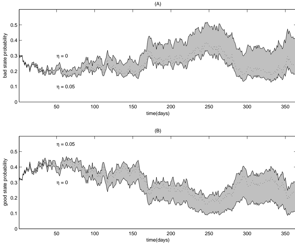
Figure 6. The effect of ambiguity aversion on the prevailing posterior probabilities dynamics. We assume three possible states and the filtered probabilities dynamics in equation (38) with parameters set equal to \sigma_D = 0.0375 , \sigma_e = 0.015 , \Theta = \{0.0023, 0.0173, 0.0323\} , \theta = 0.0173 , and a set of discretized normal priors \Pi(0) = \{0.3085, 0.3829, 0.3085\} . Panel (A) plots the probability dynamics of the "bad" state \theta_1 for three different levels of a homogenous ambiguity parameter \eta = \{0, 0.025, 0.05\} . The dynamics under the intermediate level of ambiguity \eta = 0.025 are represented by the dotted line. In Panel (B), we plot the dynamics of the posterior probabilities for the "good" state \theta_3 for the same levels of ambiguity (these graphs are based on the same random seed as the one used in Panel (A)).
