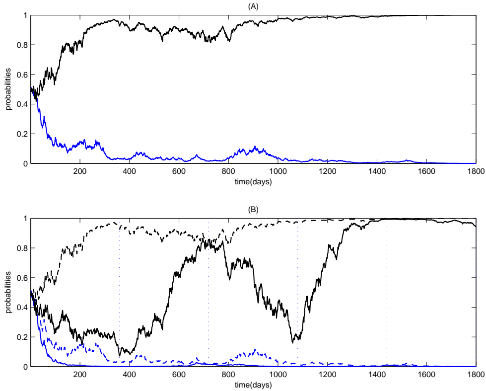
Figure 1. Posterior probabilities dynamics. The panels display trajectories for the probability \pi_1 given in equation (16) of Example 8. Panel (A) shows two trajectories for \pi_1 with a = 0 in equation (17). We plot the same trajectories with the same random seed in Panel (B) (dashed lines) and add the trajectories (solid lines) where we assume a = 0.015 . The switching in equation (17) is deterministic and occurs every year (see the dotted vertical lines in Panel (B)). The further parameters are \Theta = \{0.0075, 0.0275\} , \sigma_D = 0.0375 , \sigma_e = 0.015 .
