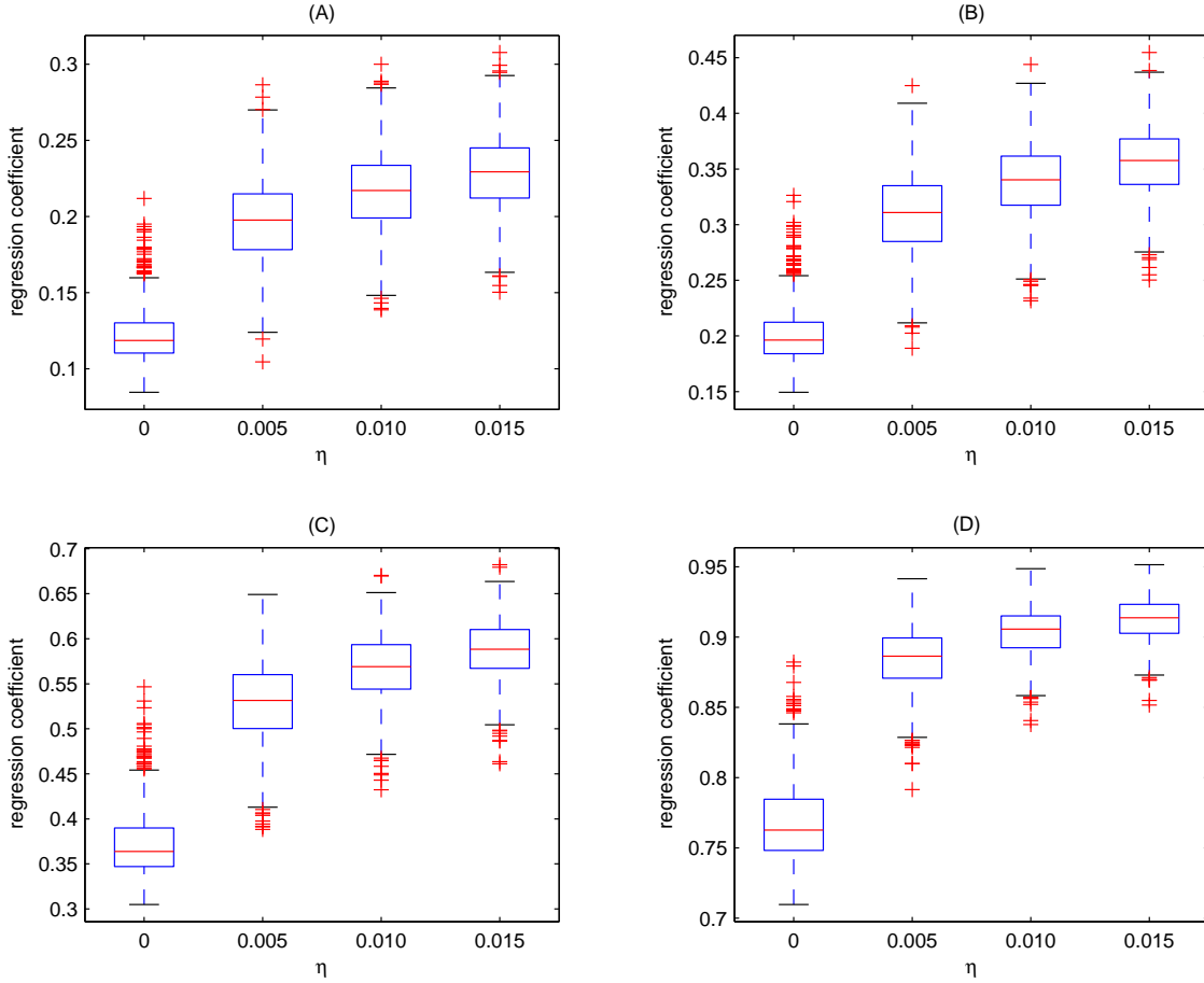
Figure 11. Regression analysis. For different parameters \gamma = 0.3, 0.5, 0.7, 0.9 , we present the box plots of the estimated parameters in 1000 regressions of dD/D on dP/P + P/D . The regressions are based on sample sizes of 365 observations simulated from a model with three reference model drift states \Theta = \{0.0025, 0.0175, 0.0325\} and under three homogenous degrees of ambiguity \eta = 0, 0.005, 0.01, 0.015 . The true dividend is \theta = 0.0175 . Further parameters are \delta = 0.05 , \sigma_D = 0.0375 , \sigma_e = 0.015 .
