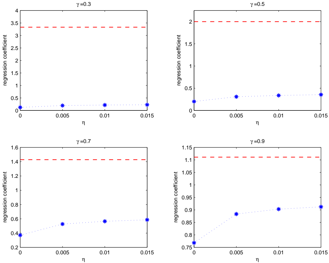
Fig. 10. Regression analysis. For different parameters \gamma = 0.3, 0.5, 0.7, 0.9 , we plot the mean estimated parameter in 1000 regressions of dD/D on dP/P + P/D . The regressions are based on sample sizes of 365 observations simulated from a model with three reference model drift states \Theta = \{0.0025, 0.0175, 0.0325\} and under three homogenous degrees of ambiguity \eta = 0, 0.005, 0.01, 0.015 . The true dividend is \theta = 0.0175 . Further parameters are \delta = 0.05 , \sigma_D = 0.0375 , \sigma_e = 0.015 . In all panels, the dashed horizontal lines give the correct underlying value 1/\gamma of the EIS. The dotted lines give the resulting mean parameter estimates as a function of \eta .
