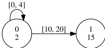
Figure 1: An example of a RAG. The leftmost state is the start state. Every state transition contains a guard. Missing transitions lead to the start state. Every state contains an identification number (above) and a prediction value (below).
