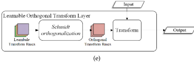
Fig. 7. Constructing the FDIT layer with IDCT, IDWT, IDFT and LNT.
