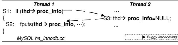
Figure 1. An atomicity violation bug from MySQL.
