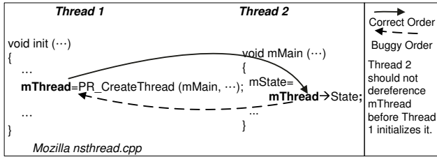
Figure 2. An order violation bug from Mozilla. The program fails to enforce the programmer’s order intention: thread 2 should not read mThread until thread 1 initializes mThread . Note that, this bug could be fixed by making PR_CreateThread atomic with the write to mThread . However, our bug pattern categorization is based on root cause, regardless of possible fix strategies.
