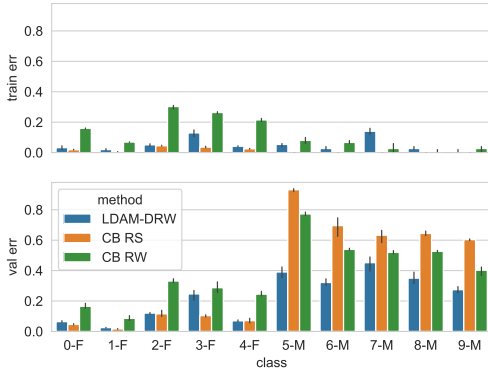
Figure 2: Per-class top-1 error on CIFAR-10 with step imbalance ( \rho = 100, \mu = 0.5 ). Classes 0-F to 4-F are frequent classes, and the rest are minority classes. Under this extremely imbalanced setting RW suffers from under-fitting, while RS over-fits on minority examples. On the contrary, the proposed algorithm exhibits great generalization on minority classes while keeping the performance on frequent classes almost unaffected. This suggests we succeeded in regularizing minority classes more strongly.
