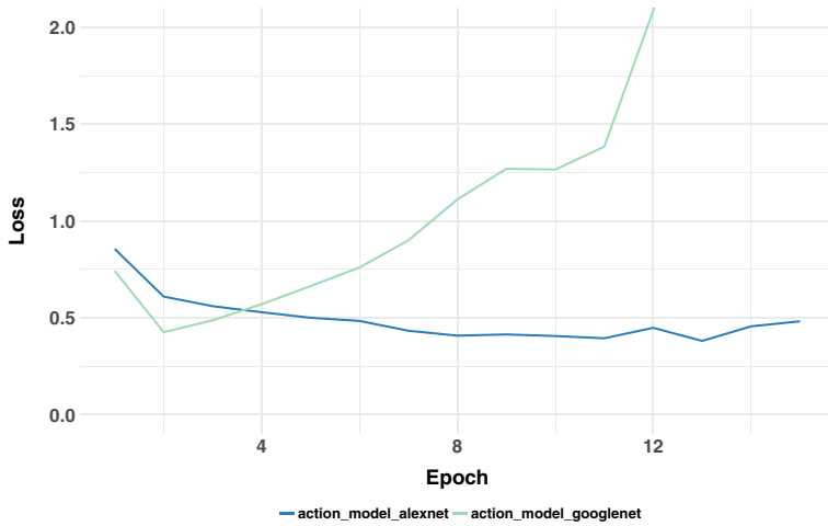
(a) Loss
