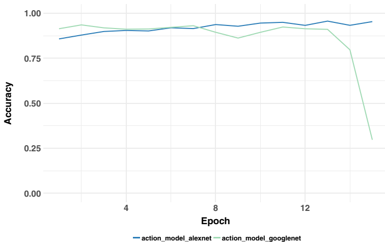
(b) Accuracy
