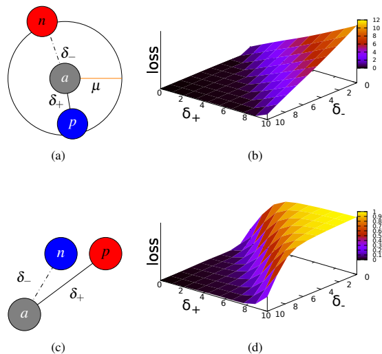
Figure 1: (a) The margin ranking loss seeks to push \mathbf{n} outside the circle defined by the margin \mu , and pull \mathbf{p} inside. (b) Margin ranking loss values in function of \delta_-, \delta_+ (c) The ratio loss seeks to force \delta_+ to be much smaller than \delta_- . (d) Ratio loss values in function of \delta_-, \delta_+ .
