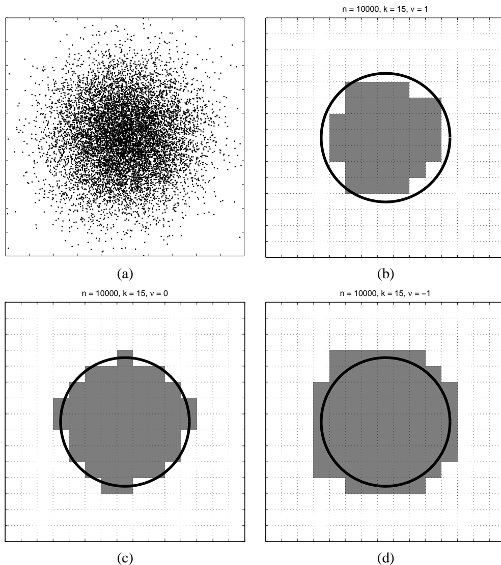
Figure 4: Data and three representative MV-ERM histogram estimates for the data in Section 7.1. The shaded region is the MV-set estimate, and the solid circle indicates the true MV-set. All estimates are based on the Occam bound. (a) 10000 realizations used for training. (b) MV-ERM estimate with a bin-width of 1/15 and v = 1 . (c) v = 0 . (d) v = -1 . Clearly, the larger v , the smaller the estimate.
