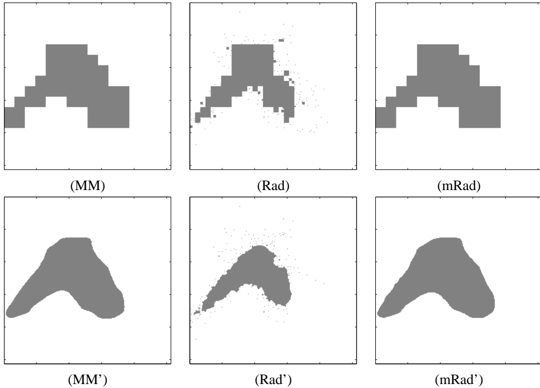
Figure 9: Minimum volume set estimates based on dyadic quadrees for \alpha = 0.90 with n = 1000 samples. Reconstructions based on MM = minimax penalty (23), Rad = Rademacher penalty (24), and mRad = modified Rademacher penalty (25), and MM', Rad', and mRad' denote the analogous estimates based on voting over multiple trees at different shifts.
