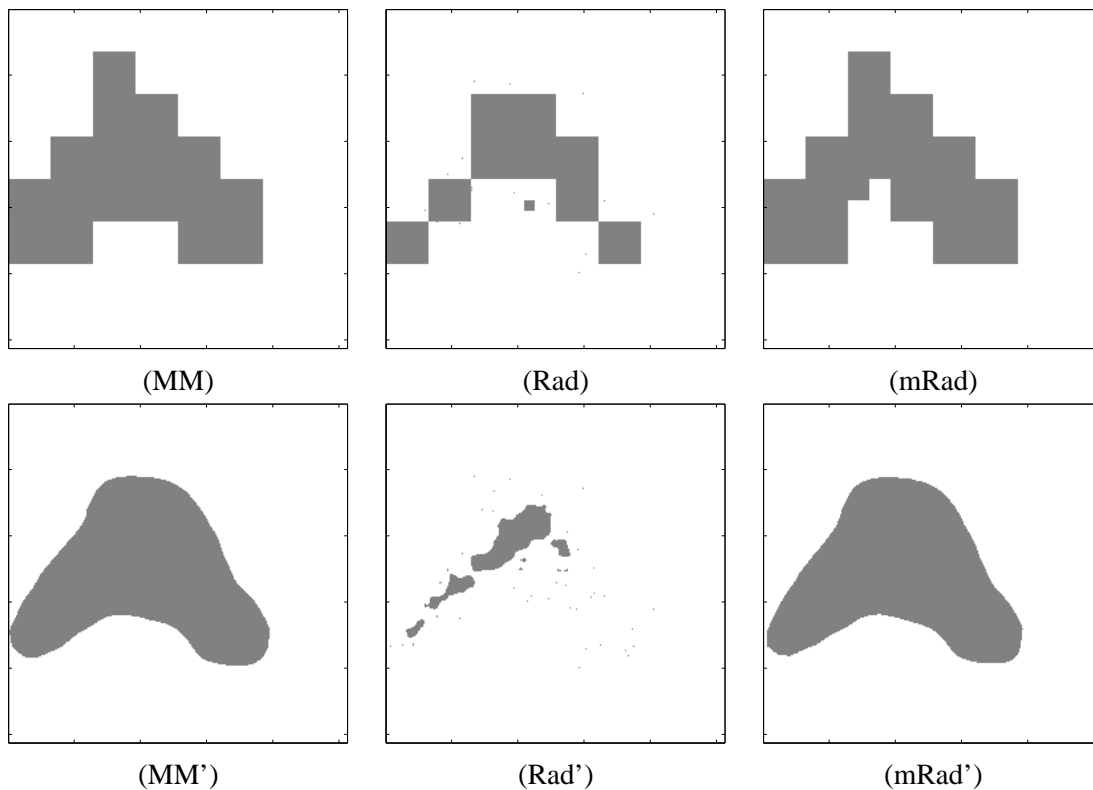
Figure 8: Minimum volume set estimates based on dyadic quadtrees for \alpha = 0.90 with n = 100 samples. Reconstructions based on MM = minimax penalty (23), Rad = Rademacher penalty (24), and mRad = modified Rademacher penalty (25), and MM', Rad', and mRad' denote the analogous estimates based on voting over multiple trees at different shifts.
