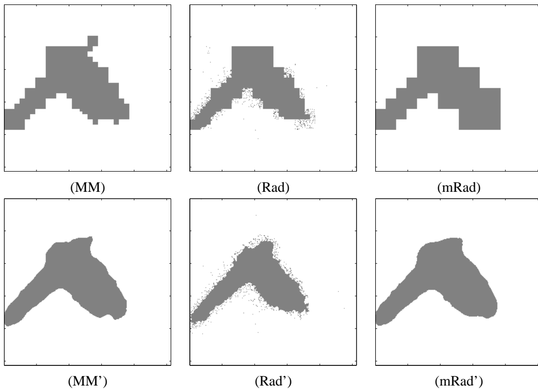
Figure 10: Minimum volume set estimates based on dyadic quadrees for \alpha = 0.90 with n = 10000 samples. Reconstructions based on MM = minimax penalty (23), Rad = Rademacher penalty (24), and mRad = modified Rademacher penalty (25), and MM', Rad', and mRad' denote the analogous estimates based on voting over multiple trees at different shifts.
