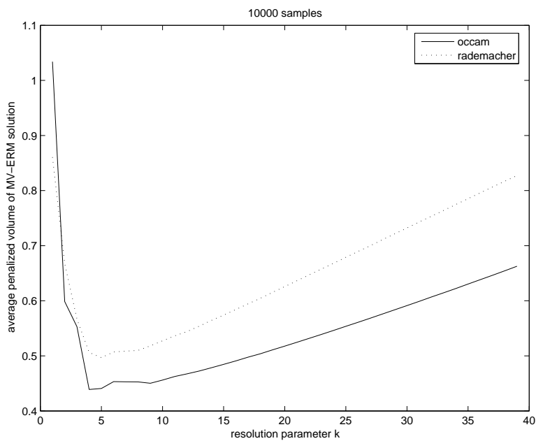
Figure 6: The penalized volume of the MV-ERM estimates G_{\hat{G},\alpha}^k , as a function of k , where 1/k is the sidelength of the histogram cell. The results are for a sample size of 10000. Results represent an average over 100 repetitions. Clearly, the Occam's razor bound is smaller than the Rademacher penalty (look at the right side of the plot), to which we may attribute its improved performance (see Figure 5).
