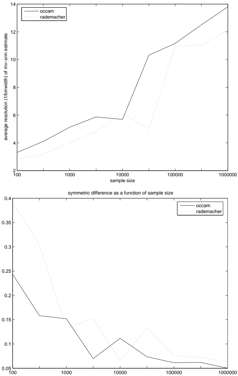
Figure 7: Results from the histogram experiments in Section 7.1. All results are averaged over 100 repetitions for each training sample size, and are for the non-damped version of MV-SRM ( v = 1 ). (Top) Average value of the resolution parameter k ( 1/k = sidelength of histogram cells) as a function of sample size. (Bottom) Average value of the symmetric difference between the estimated and true MV-sets. Neither graph changes significantly if v is varied.
