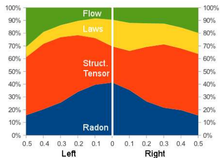
Fig. 5. Breakdown of the contribution of the different features for different control prediction strengths, averaged over 9389 datapoints. Laws and Radon are more significant in cases where small controls are performed (e.g. empty scenes), whereas the structure tensor and optical flow are responsible for strong controls (e.g. in cases where the scene contains an imminent obstacle). A slight bias to the left can be seen, which is consistent to observations in the field. Best viewed in color.
