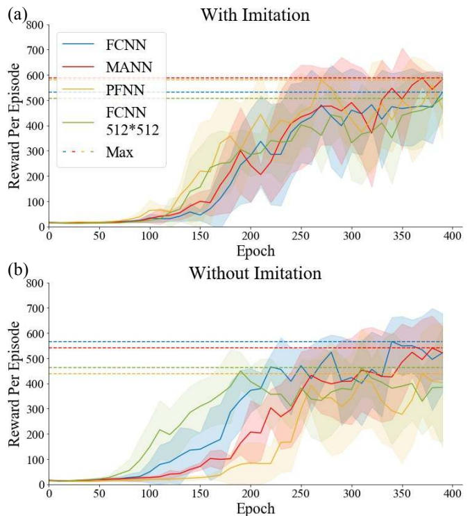
Fig. 5: Learning curve for 4 different network setups averaged over 5 trials.
