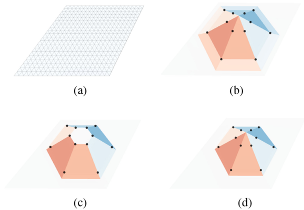
FIGURE 6. Solutions of the minimum-norm interpolation problem.
