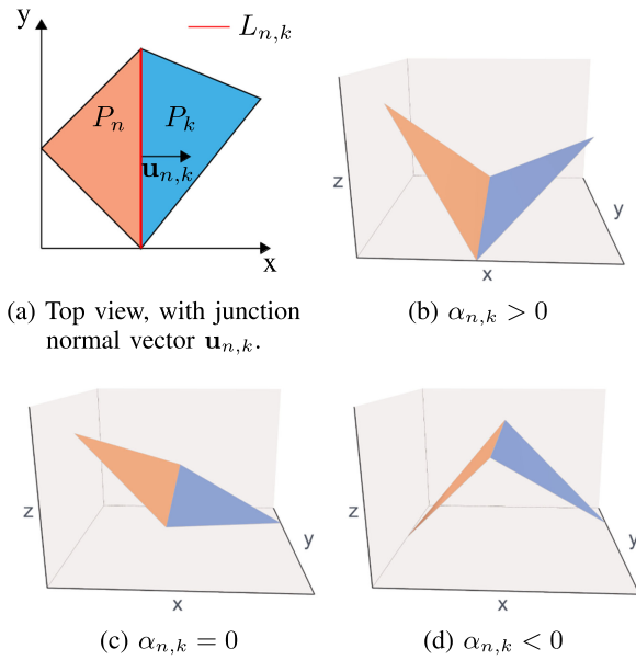
FIGURE 1. \alpha_{n,k} for different junctions.
