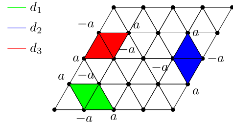
FIGURE 5. Convolutional filters; a = \frac{2\sqrt{3}}{3} .
