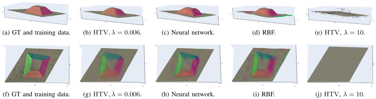
FIGURE 7. HTV regularization vs. ReLU neural network vs. radial basis functions.
