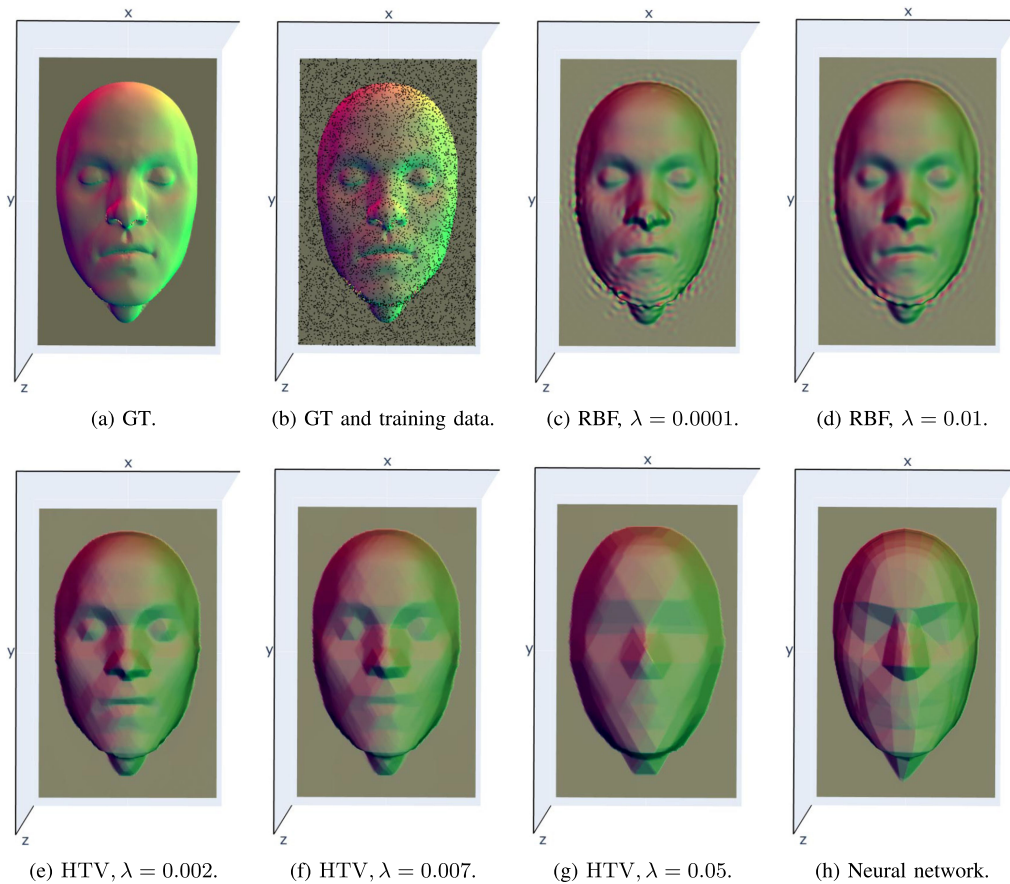
FIGURE 8. HTV regularization vs. ReLU neural network vs. radial basis functions.
