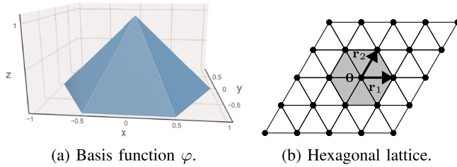
FIGURE 3. Principal elements of our search space.
