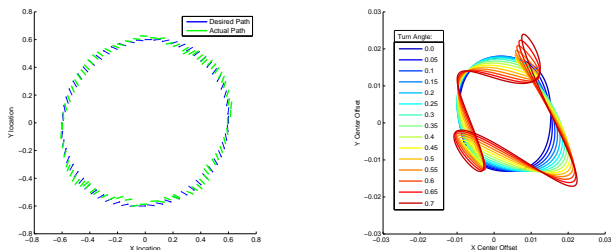
(a) Desired and actual trajectories for the learned controller on path 1. (b) Parametric center offset curves for several different turning angles.
