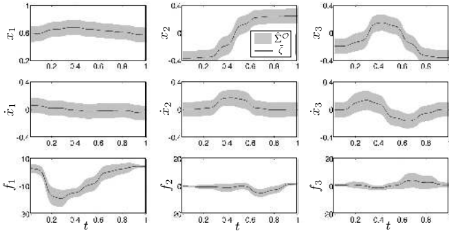
Fig. 4: Estimated desired state of the robot \bar{\zeta} and its associated variance \bar{\Sigma}^o along a reproduction of the cooperative transportation. Position, velocity and forces are respectively given in meters, meters per second, and Newtons.
