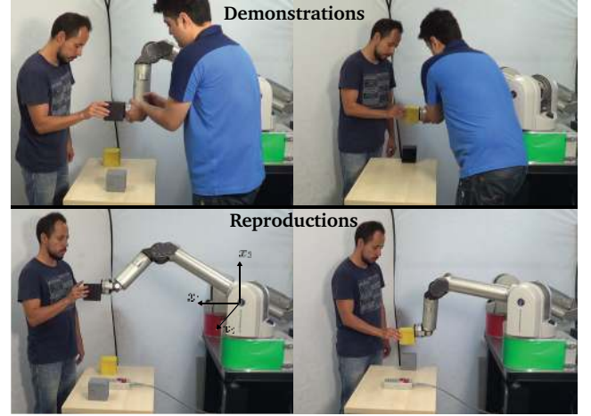
Fig. 2: Experimental setting of the human-robot transportation task: (top) kinesthetic demonstrations, and (bottom) reproduction phase.
