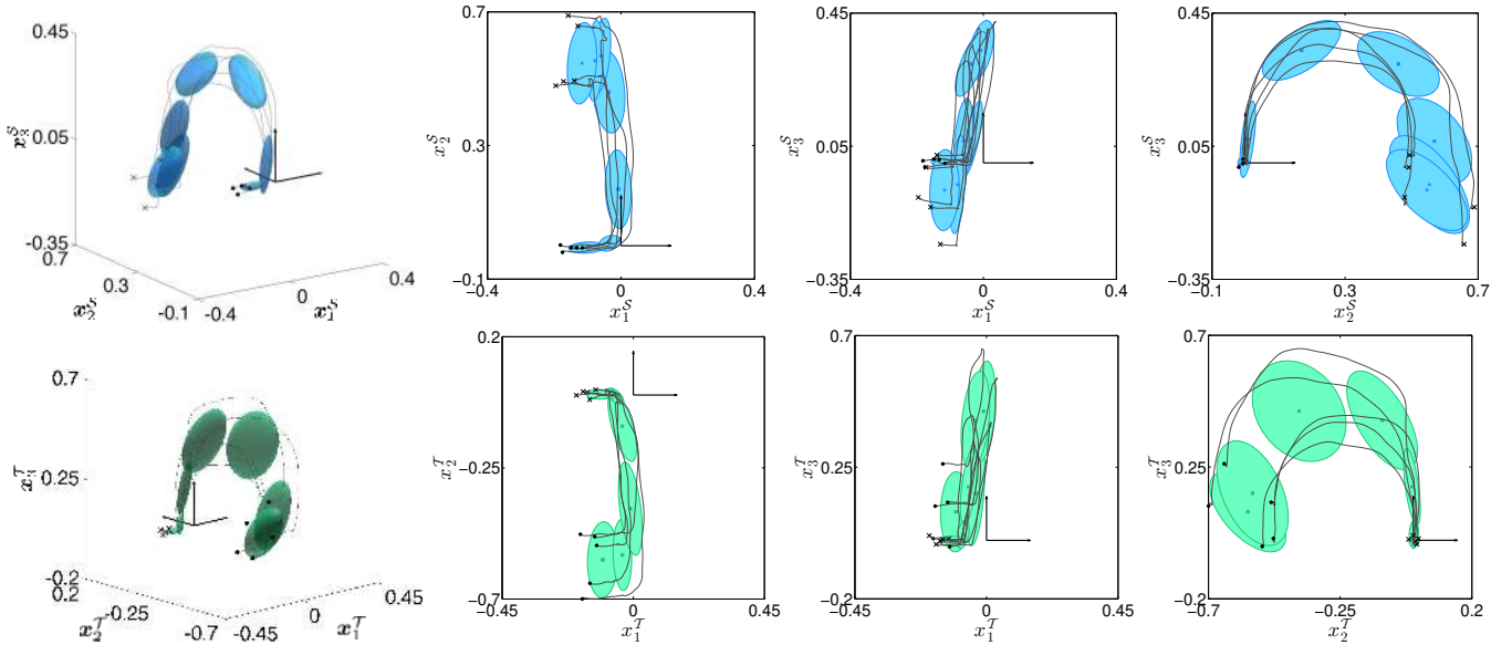
Fig. 3: Encoding of the demonstrations in the different coordinate systems. The local models in the start and target frames are respectively shown in the first and second rows (projected on the position subspace of the data). The gray lines depict the end-effector trajectory (in meters) observed from the different frames. The ellipsoids represent the Gaussian components of the model. Black dots depict the beginning of the demonstration.
