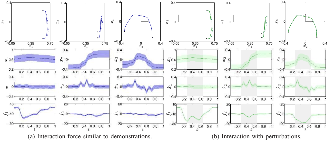
Fig. 7: Reproductions of the cooperative transportation. The first row shows the robot trajectory (solid line) and the desired path (dashed line) in the three planes of the Cartesian space. The remaining rows show the position, velocity and sensed force of the robot over time (solid lines), along with corresponding feedback gain (represented as an envelope surrounding the reproduced trajectory).
