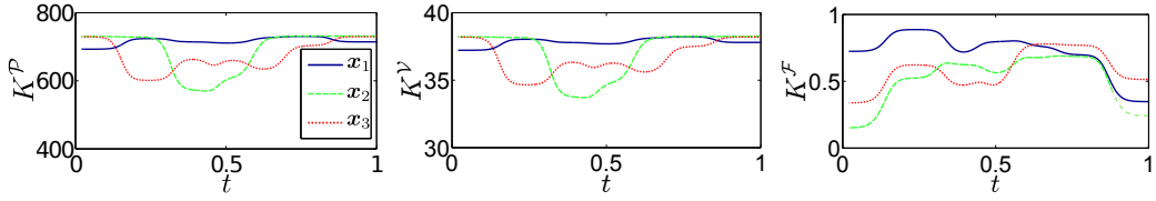
Fig. 6: Profiles of the diagonal values of the estimated stiffness, damping and force gain matrices during the reproduction of the cooperative transportation.
