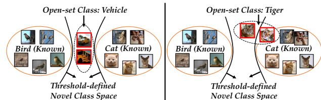
Figure 1. The drawback of threshold-based open-set recognition. It defines novel class space if confidence below a fixed threshold. Bird and cat are known classes, while vehicle and tiger are open-set classes in the left and right figures, respectively. Since the distributions of the vehicle and tiger categories differ, it is hard to rely on a single threshold to recognize unknown classes with diverse characteristics. The same threshold which well separates vehicles apart from known classes is not suitable for tigers.
