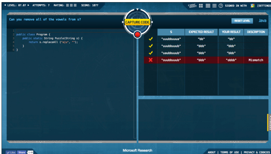
Fig. 9. The main window of Code Hunt is split into two parts: the left part shows the code being run and the right part shows the result of the execution of the public tests.
