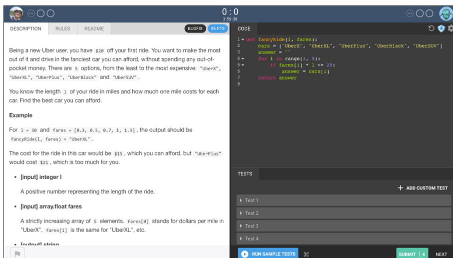
Fig. 10. The main window of Code Fights is split into two parts: the left part shows the statement of the challenge and the right part shows the code and the result of the execution of the public tests.
