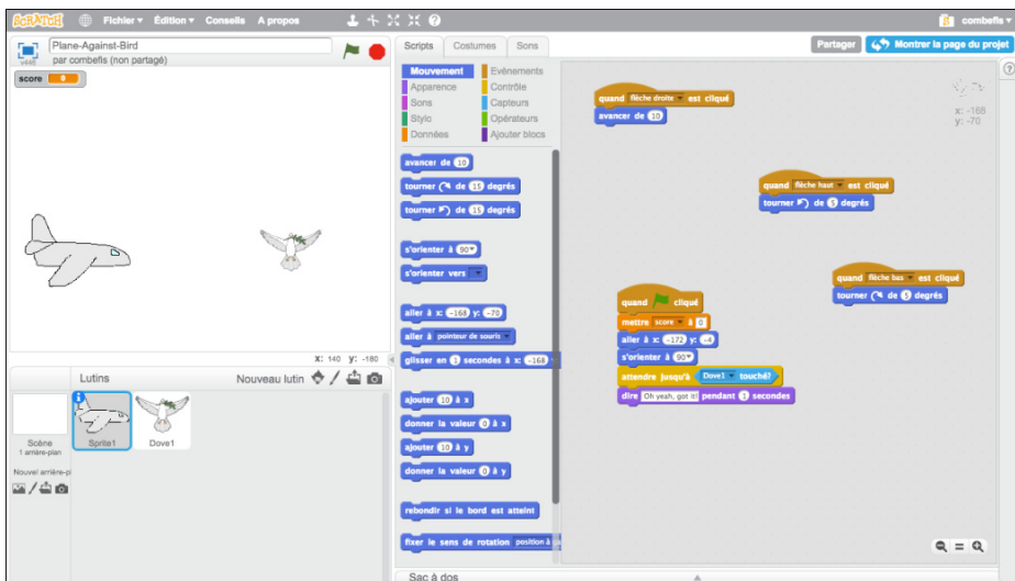
Fig. 5. The main window of the Scratch program is split into two parts: the left part shows the sprites of the game and the right part shows the programs representing the behaviour of the different sprites.
