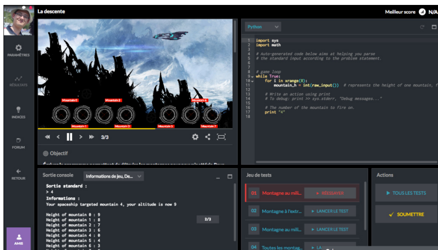
Fig. 8. In this mission, the agent is a spaceship that must destroy targets on the ground. These targets have different heights so that the spaceship must destroy them in the right order if it does not want to enter in collision with any of them.
