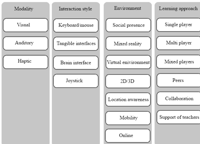
Fig.1. The classification of the educational programming games (adapted and extended schema of Laamarti et al. , 2014).
