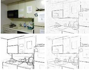
Fig. 2. Qualitative comparison of contours: Top row: color image, contours from [9], bottom row: contours from [18] and contours from our proposed contour detector
